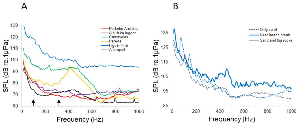
Fig. 3. Ambient noise in the recording locations. A - Average sound power spectra of ambient noise from the different studied locations (1-3 sites within each location). B depicts the sound spectra from three different recording sites at Figueirinha beach. Note the peak at around 450 Hz in the recording near the beach break, delimiting an area with sand substrate. Arrows depict an AN quiet window.
