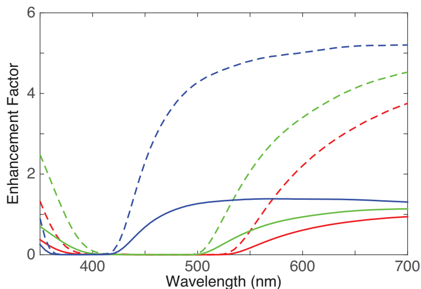
Fig S3: Calculations of enhancement with and without outer segments as a comparison to the Mie scattering calculations of Ives et al. (1983) for the receptor geometry, refractive indices and oil droplet absorption spectra of the turtle Trachemys scripta elegans . Solid lines show enhancement factors including the outer segment and dashed lines show calculations without. When the outer segment is not present we recover greater enhancement factors that approach those calculated by Ives et al. (1983). This is due to the waveguiding effect of the outer segment, which allows it to confine light to its volume even without the presence of the oil droplet. Red lines – LWS cone. Green lines – MWS cone. Blue lines – SWS cone.
