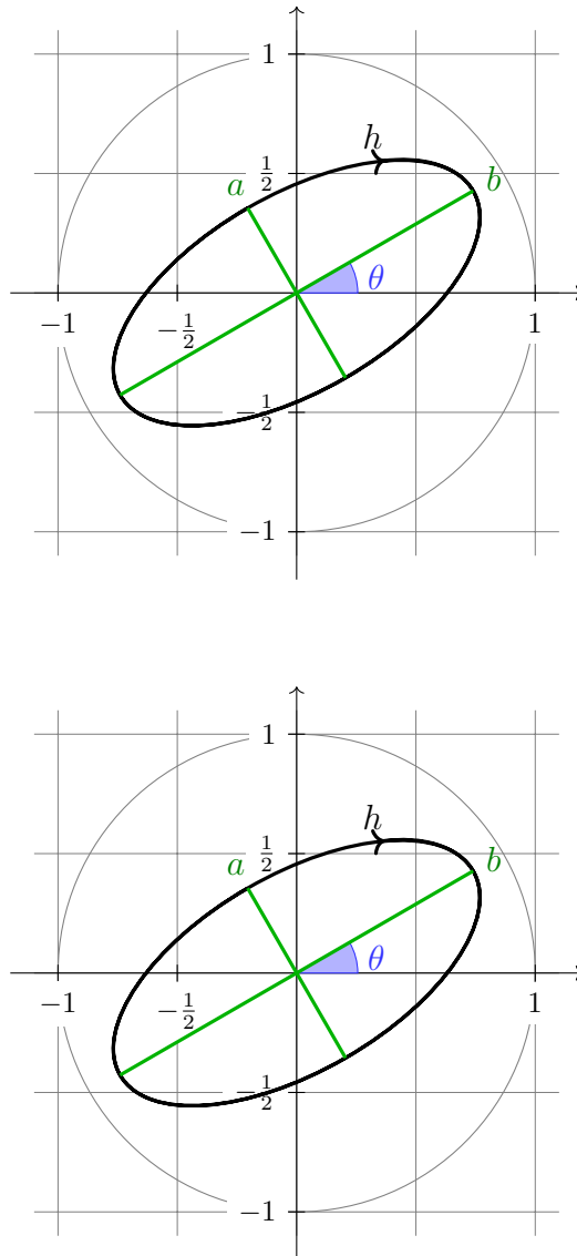
Figure 1: The polarization ellipse of partly polarized light: Here, the Stokes parameters [s_1, s_2, s_3] are equal to [0.15, 0.26, 0.8] (arbitrary chosen values) respectively. Using Equations 3–7, we can calculate that the total polarization is 85%, the angle of polarization is 30^\circ , and the two axes are 0.41 and 0.85. The handedness of the light is indicated by the clockwise turning arrow (the light is right-hand circularly polarized). Notice that since the sum of squares of these stoke parameters must be smaller (or equal) to the square of the first Stokes parameter, the ellipse can never be larger than the grey circle (with a radius equal to one).
