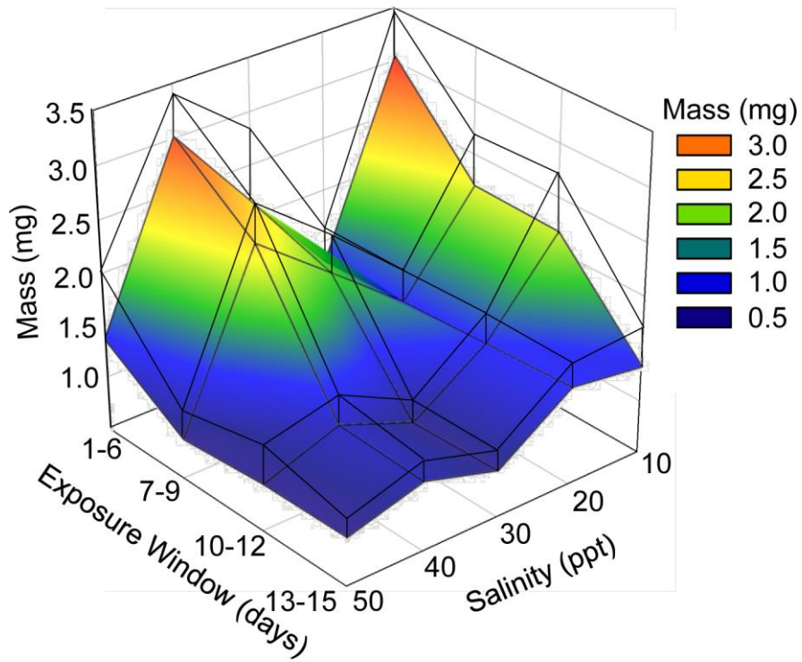
Fig. 6. 3-D graph with error overlay. Mean mass (mg) of Artemia franciscana on day 15 as in Fig. 2B with an overlay (dark lines) created from s.e.m. for each treatment.
