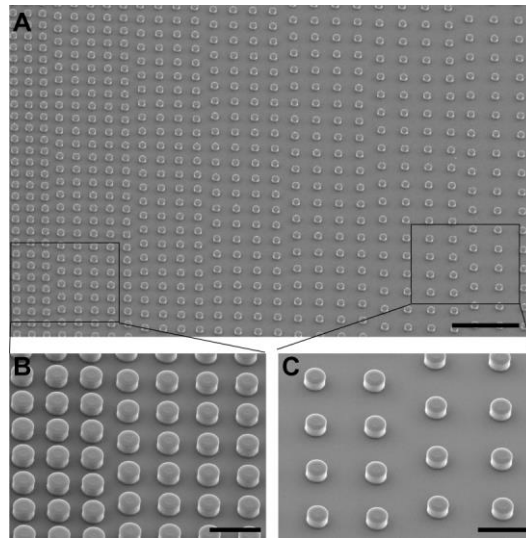
Fig. 1. SEM micrographs of the transparent ‘gradient’ microstructured epoxy substrate with square arrays of cylindrical pillars 1.4 \mu\text{m} in height and 2 \mu\text{m} in diameter. (a) from left to right, the centre-to-centre spacing increases from 3.5 to 6.5 \mu\text{m} in steps of 0.5 \mu\text{m} . (b) transition from 3.5 to 4.0 \mu\text{m} spacing. (c) transition from 6.0 to 6.5 \mu\text{m} spacing. Scale bars: 20 \mu\text{m} (a), and 5 \mu\text{m} (b, c).
