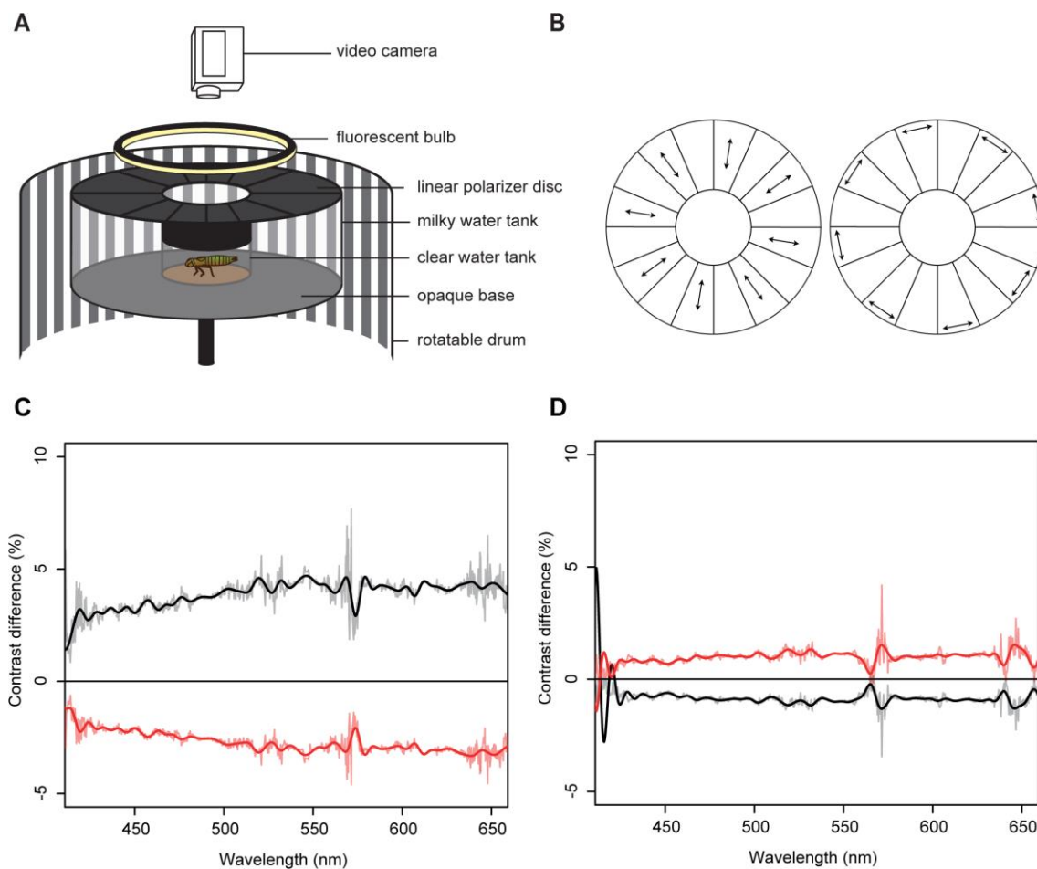
Fig. 4. Experimental apparatus used to test the optomotor response and the changes in contrast of the square-wave gratings when polarization filtering was applied. A: Experimental set up to test the optomotor response of dragonfly larvae to a moving square-wave grating of vertical stripes. The subject animal was contained in the stationary central cylinder of clear water, which was surrounded by a concentric outer tank containing dilute milk solution. Light to the latter, from above, was polarized by one of two linear polarizing discs (B), consisting of radially or tangentially orientated linear polarizers, resulting in vertically or horizontally polarized light (respectively) being scattered towards the subject. This veiling light field reduced the contrast of the grating, which was fixed to a rotatable outer drum. The animal's response was assessed by their measuring their ability to visually track the rotation of the grating. B: Polarizer discs used to change the polarization of the light illuminating the milky water tank, constructed of sectors of Polaroid™ filter. The arrows indicate the transmission axis of the linear polarizer in each sector. Two light fields were created using these discs independently: one vertically polarized (left disc), and the other horizontally polarized (right disc). C and D: Change in intensity contrast of the grating stripes, from measurements made without a linear polarizer, when measurements were made
