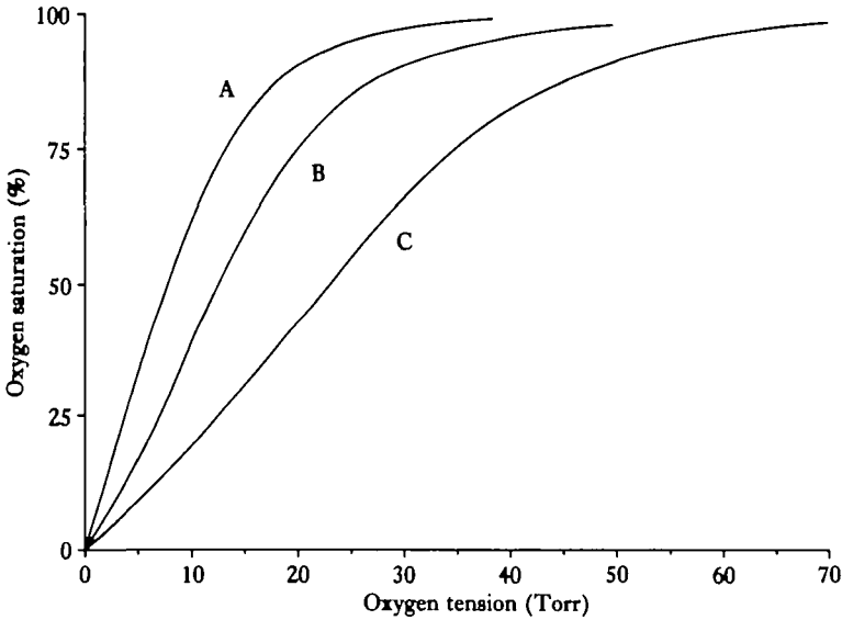
Fig. 1. Oxygen equilibrium curves of mid-gestation foetal (A), late-gestation foetal (B) and adult (C) bloods in the absence of exogenous \text{CO}_2 .
