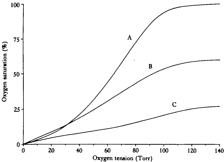
Fig. 2. Oxygen equilibrium curves as in Fig. 1 in the presence of 5.6% \text{CO}_2 .
