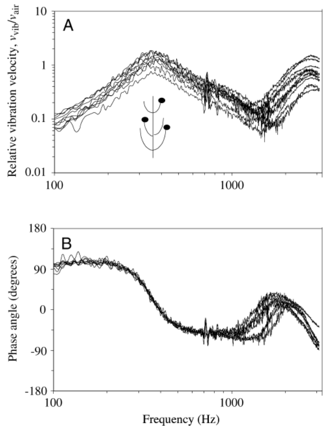
Fig. 9. Frequency responses measured at the tips of different hairs inserting at different heights on the same male antenna. The magnitude (A) and phase (B) of the antennal vibration velocity v_{\text{vib}} relative to the particle velocity v_{\text{air}} .
