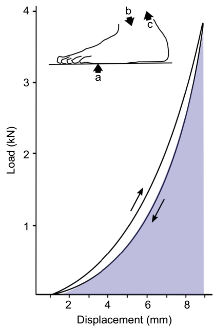
Fig. 7. Elastic energy storage and release in the human foot. Force–displacement curve modified from Ker et al. (1987) for a cadaveric foot under a simulated load at midstance for a 70 kg person running at 4.5 m s -1 . A load was applied to the base of the foot using an actuator to simulate ground reaction force (a) and triceps surae force (b), resulting in the total compressive force on the arch (c). Arch displacement was measured as the displacement of the actuator. As force is applied, the arch deforms (upward arrows) and then recoils (downward arrows), losing some energy (area between the curves), but returning most energy (shaded blue region under the curve).
