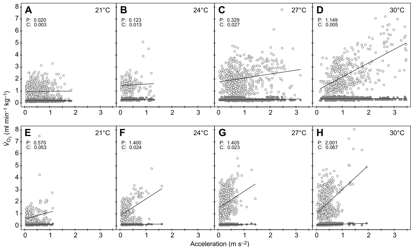
Fig. 3. Effect of activity levels (body acceleration) on bimodal oxygen consumption rates over the four temperature treatments. (A–D) Hydrophis curtus and (E–H) H. elegans . Open circles with trendlines represent relationships between \dot{V}_{O_{2,pul}} and body acceleration, and filled circles with trendlines represent relationships between \dot{V}_{O_{2,cut}} and body acceleration. The slope of each relationship is displayed in each plot (P, pulmonary; C, cutaneous).
