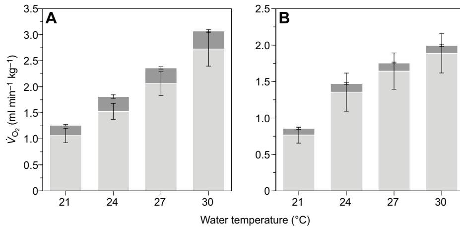
Fig. 2. Patterns in mean oxygen consumption rate via pulmonary ( \dot{V}_{O_{2,pul}} ) and cutaneous ( \dot{V}_{O_{2,cut}} ) pathways across the four temperature treatments. \dot{V}_{O_{2,pul}} , light grey; \dot{V}_{O_{2,cut}} , dark grey. (A) Hydrophis curtus ( N=11 ) and (B) H. elegans ( N=10 ). Note the difference in scale of the vertical axes, whereby the absolute values are consistently higher for H. curtus . Mean values are displayed \pm s.e.m.
