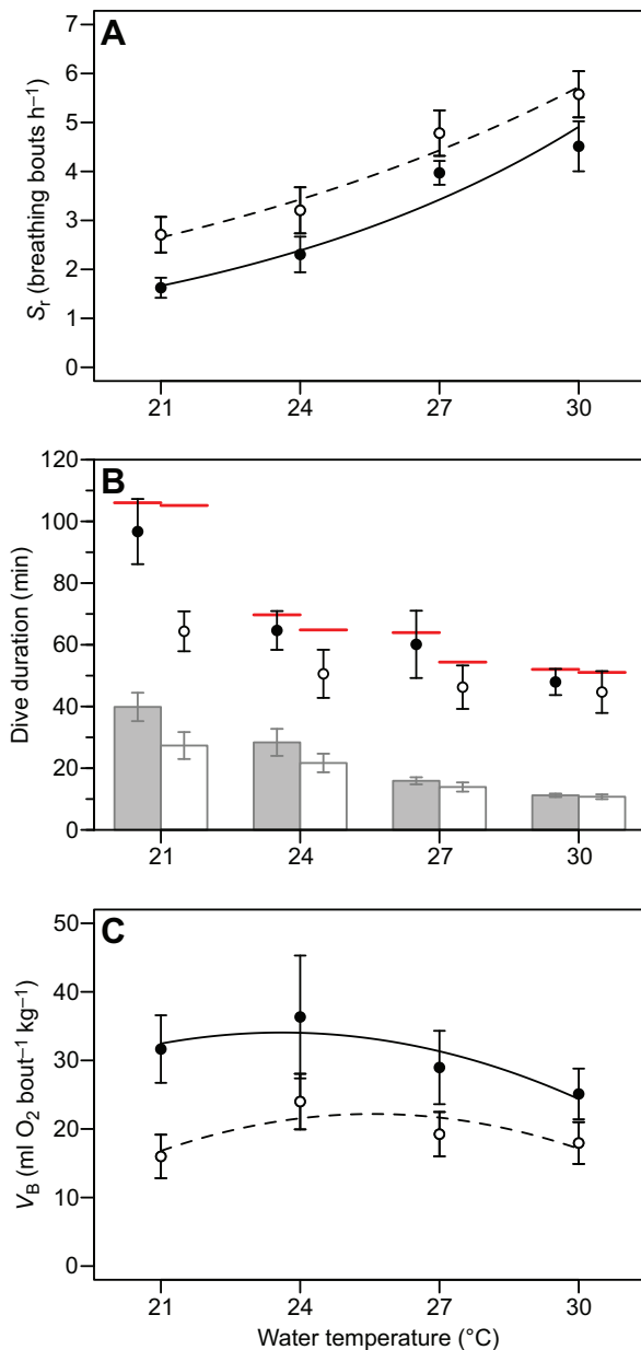
Fig. 1. Metrics of dive behaviours of Hydrophis curtus and Hydrophis elegans . Hydrophis curtus : filled circles and bars ( N=11 ); H. elegans : open circles and bars ( N=10 ). (A) Increased surfacing rate ( S_r ) with increased water temperature. (B) Decreasing mean dive duration with increasing temperature (bar plot). Points represent mean maximum dive durations among all observed individuals, with red lines indicating theoretical maximum aerobic dive duration. (C) Relatively constant oxygen consumption per breathing bout ( V_B ) across temperatures. Mean values are displayed \pm s.e.m.
