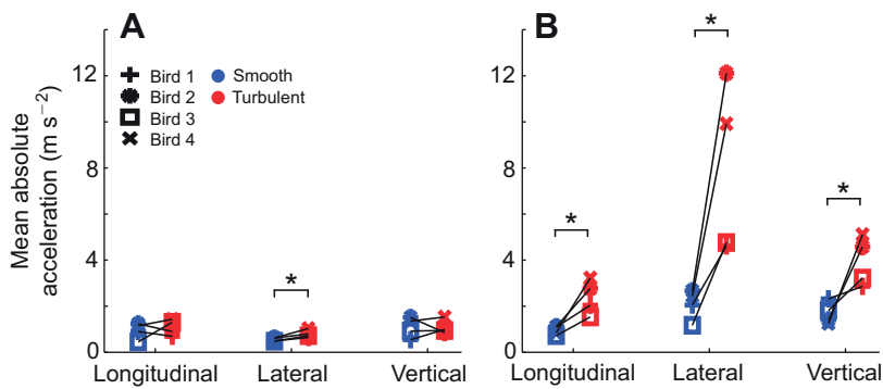
Fig. 2. Mean absolute accelerations experienced by ruby-throated hummingbirds. Absolute acceleration on (A) the head and (B) the body along the longitudinal, lateral and vertical directions of the wind tunnel in smooth (blue) and turbulent (red) flow conditions. * P < 0.05 .
