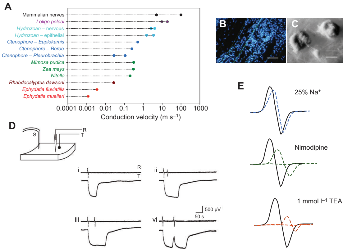
Fig. 4. Electrical conduction in glass sponges. (A) Conduction velocities in plants and animals. (B) Microtubules (green) and nuclei (blue) in giant syncytia of the glass sponge Rhabdocalyptus dawsoni . (C) Adherent aggregates fusing with the syncytial tissue of R. dawsoni , a preparation that allows extracellular recording from the sponge. (D) Diagram of the recording setup and records of action potentials in R. dawsoni (from Leys et al., 1999). S, stimulating electrode; R, recording electrode; T, thermistor flow probe. Top traces, electrical records; bottom traces, thermistor flow records: (i) a single stimulus causes an AP and arrest of flow; (ii,iii) repeated stimuli cause further APs even though the flow is still arrested; (iv) after pumping resumes a second stimulus causes a second AP and arrests the flow again. (E) Effect of sodium, calcium and potassium on the action potential in R. dawsoni (after Leys et al., 1999). Top, 75% reduction of sodium (replacement with choline chloride); middle, the calcium blocker nimodipine (24 \mu\text{mol l}^{-1} ) delays and blocks the AP, reversibly; bottom, the potassium channel blocker TEA reduces, delays and then blocks the AP, also reversibly. Scale bars: 20 \mu\text{m} (B); 1 mm (C).
