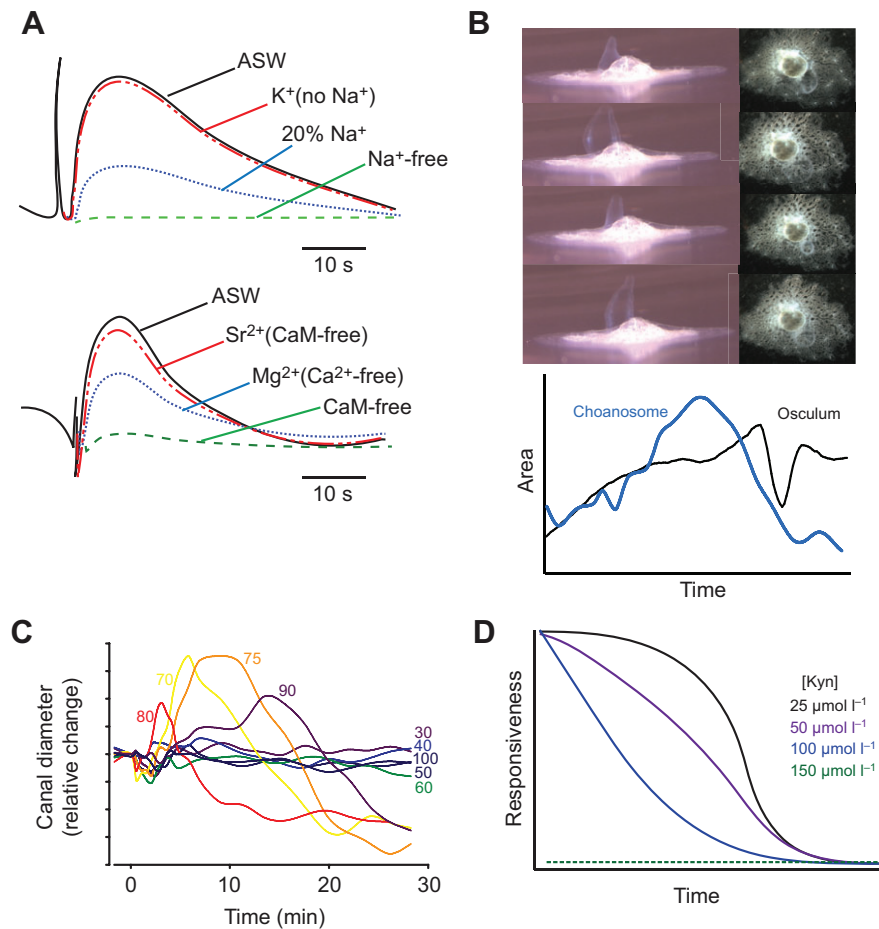
Fig. 3. Ionic basis of contractions in freshwater sponges. (A) Substitution of sodium (top panel) and calcium and magnesium (bottom panel) in marine sponges (after Prosser, 1967). Solid line (both panels): ASW control. Top panel: dotted blue line, 80% reduction in sodium (sodium replaced with sucrose); dashed green line, no sodium, 100% sucrose; dash-dotted red line, potassium instead of sodium. Bottom panel: dotted blue line, magnesium but no calcium; dashed green line, neither calcium nor magnesium; dash-dotted red line, strontium instead of calcium and magnesium. (B) Contraction of the osculum (left) and choanosomal region with feeding chambers (right) of Ephydatia muelleri with tracings showing the time of both events below. (C) Concentration-dependent effect of glutamate on the inflation–contraction behaviour of E. muelleri . A full ‘sneeze’ is triggered by 75 \mu\text{mol l}^{-1} L-Glu; lower concentrations generate localized contractions and higher concentrations cause the surface of the sponge to tear, whereas the canals continue a full inflation–contraction event (from Elliott and Leys, 2010). (D) Concentration-dependent effect of glutamate blocker kynurenic acid on contractions in E. muelleri . Longer incubation in Kyn reduces responsiveness to L-Glu, even at lower concentrations of the inhibitor. High concentrations of the inhibitor block all contractions.
