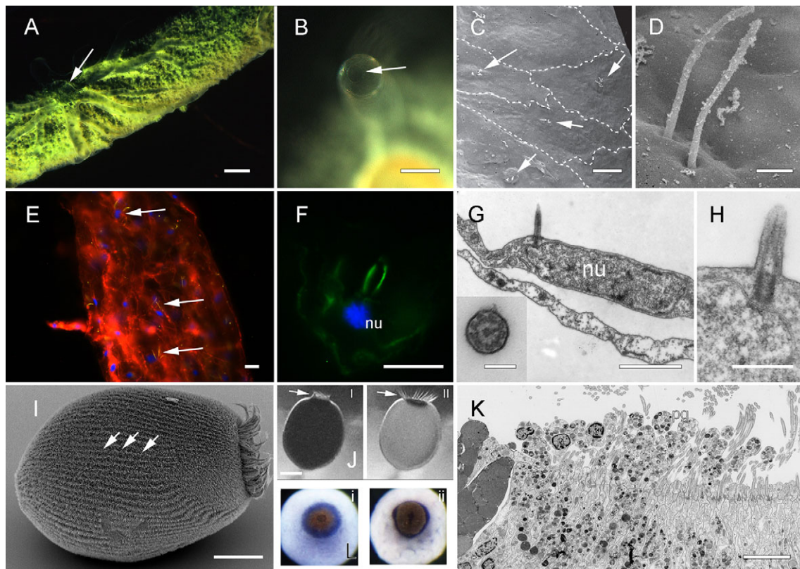
Fig. 2. Sensory cilia in sponges. (A) Transparent raised excurrent canals leading to the osculum (arrow) in Spongilla lacustris encrusting on a branch in a lake. (B) The osculum (arrow) of a small lab-hatched individual of Spongilla lacustris . (C,D) Scanning electron micrographs of cilia (arrows) on the inner epithelium of an osculum cut open lengthwise. (E,F) Immunofluorescence of the whole osculum (E), and a single endopinacocyte (F) showing cilia labelled with the styryl dye FM 1-43 (green, arrows), nuclei (blue) and actin (red) (images, D. Ludeman). (G,H) Transmission electron micrograph of a section through the osculum showing the base of one cilium arising just above the nucleus (nu); inset shows a cross section of the cilium with no clear central pair of microtubules. (I) Scanning electron micrograph of the larva of Amphimedon queenslandica showing swimming cilia forming metachronal waves (arrows) and long posterior cilia (right). (J) Response of the long posterior cilia in A. queenslandica to changes in light intensity: (I) bent when suddenly dark and (II) straightened when suddenly light (from Leys et al., 2002). (K) Transmission electron micrograph through the pigment granules (pg) and long posterior cilia of the A. queenslandica larva. (L) Expression of the AqCRY2 gene in two developmental stages (i,ii) at the posterior pole of the A. queenslandica larva (from Rivera et al., 2012). Scale bars: 5 mm (A); 50 \mu m (B); 10 \mu m (C,E,F); 1 \mu m (D); 2 \mu m (G); 100 nm (G, inset); 500 nm (H); 100 \mu m (I,J); 5 \mu m (K).
