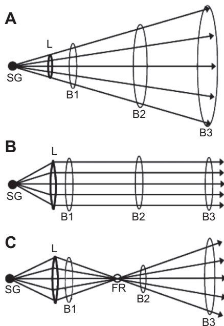
Fig. 1. Different patterns of beam attenuation with distance. (A) Unfocused beam from a point source and ideal spherical spreading. Absolute beamwidth increases with distance, but angular beamwidth remains constant. (B) Ideally focused beam in which absolute beamwidth remains constant irrespective of distance, but angular beamwidth decreases with distance. (C) Convergent beam resulting in a focal region (FR) and variable angular beamwidth measurements. SG, sound generator; L, focusing lens; B1–B3, variable beamwidths at different distances from the sound source.
