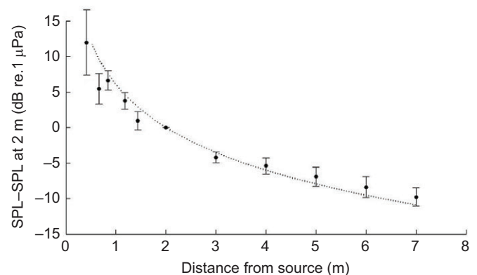
Fig. 2. Recording signals along the beam axis. See Fig. 7B for the experimental configuration. Relative sound pressure level (SPL, in dB re. 1 \mu Pa) measured at a distance from the sound source for 614 clicks from 30 click trains. The circles represent the mean difference between the SPL measured at a given distance ( r ) and the SPL measured at 2 m, and the bars represent the s.d. of each point. The dashed curve represents the spherical spreading loss function of 1/r , with a reference at 2 m.
