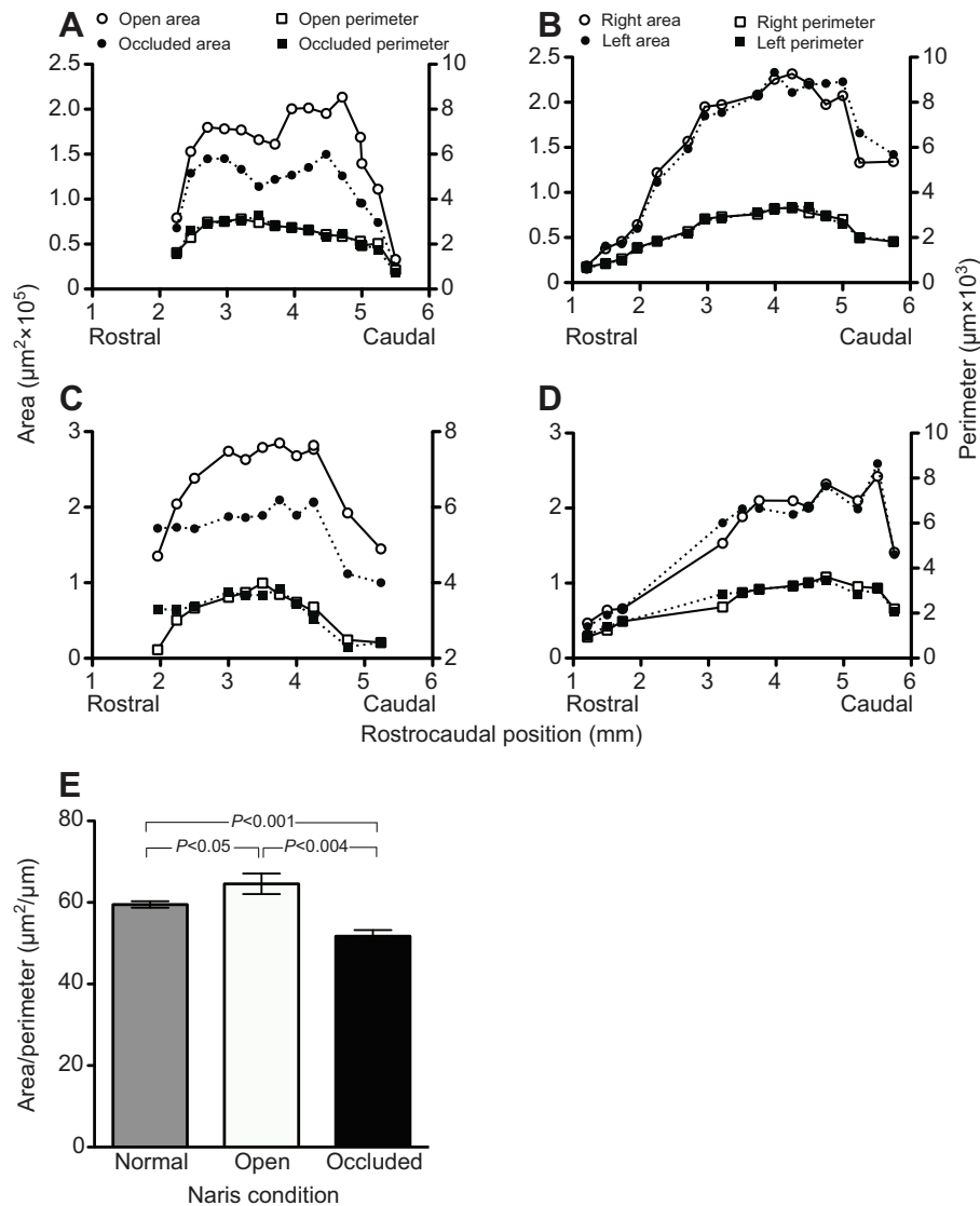
Fig. 2. Area and perimeter measurements of cross sections of Nt. (A–D) Measurements were made at different rostrocaudal positions for two UNO animals (A,C) and two normal controls (B,D). (E) Mean ( \pm s.e.m.) area/perimeter ( A/P ) group data pooled across rostrocaudal locations for occluded and open fossae ( n=7 ) as well as normal fossae ( n=4 ). Means for open and occluded fossae were compared by a paired t -test. Other comparisons were by unpaired t -test. Perimeter values alone were not significantly different between the groups.
