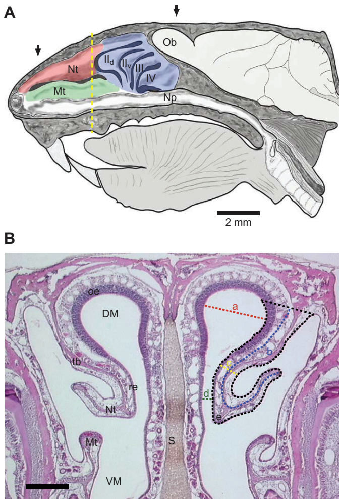
Fig. 7. Morphometric analyses. (A) Drawing of midsagittal view of murine nasal cavity with the septum removed [redrawn from Liebich (Liebich, 1975)]. Arrows mark approximate rostrocaudal limits of histological samples. Nt, nasoturbinates (red); Mt, maxilloturbinates (green); roman numerals label ethmoturbinates (blue); Np, nasopharynx; Ob, olfactory bulb. The dotted line marks the approximate location from which coronal section in B was taken. (B) Coronal section from normal (control) mouse stained with H&E illustrating morphometric measurements (dashed lines on right; see Materials and methods). a, width of dorsal meatus; b, length of turbinate; c, width of turbinate; d, turbinate-septum offset; e, perimeter of turbinate; DM, dorsal meatus; Mt, maxilloturbinates; Nt, nasoturbinates; oe, olfactory epithelium; re, respiratory epithelium; S, nasal septum; tb, turbinate bone; VM, ventral meatus. Scale bar: 300 \mu m.
