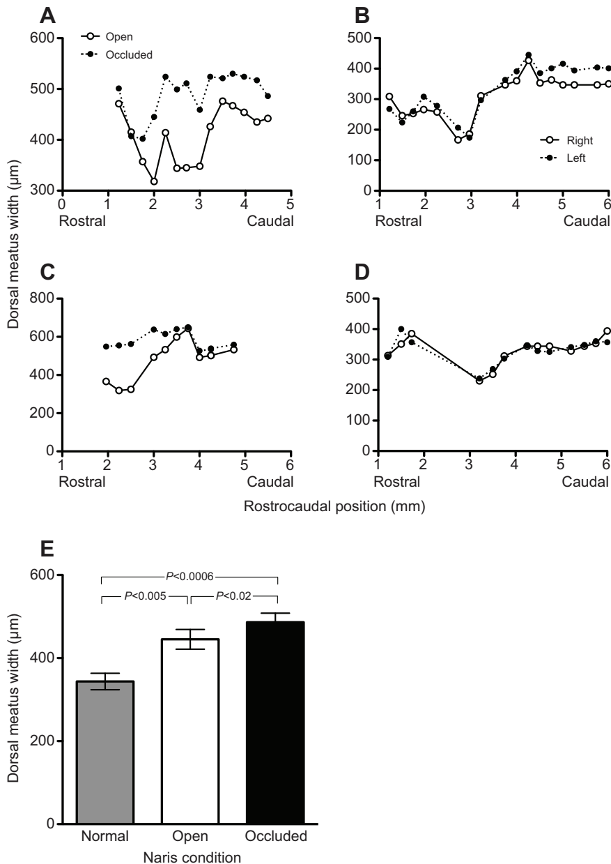
Fig. 4. Width of dorsal meatus at the inflection point. (A–D) Data from two UNO animals (A,C) and two normal controls (B,D). (E) Mean ( \pm s.e.m.) group data for width of dorsal meatus. Means for open and occluded fossae were compared by a paired t -test. Other comparisons were by unpaired t -tests. Note: occluded-side fossae are wider than open-side fossae but both are wider than controls.
