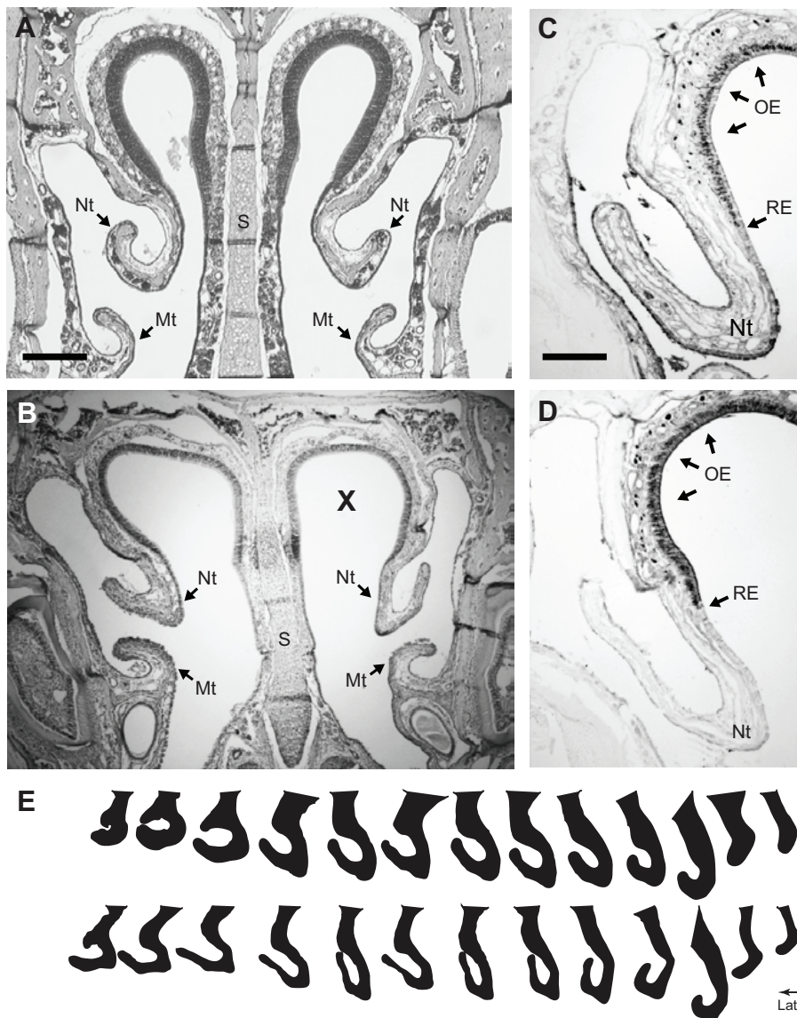
Fig. 1. Nasal anatomy. (A) Coronal H&E-stained section of a normal mouse nasal cavity showing the nasoturbinate (Nt) and maxilloturbinate (Mt). Note the remarkable symmetry of the turbinates in the two nasal fossae. (B) Similar section as A but from a UNO animal. X, occluded fossa. Note the filigree morphology of the Nt from the occluded fossa. (C) Olfactory marker protein (OMP) immunolabeling of Nt from the open fossa of a UNO mouse. (D) Same animal and label as in C but from the occluded fossa. The image has been flipped vertically to allow easier comparison of turbinate morphology. The denser OMP labeling on the occluded side, obvious in these photomicrographs, has been previously reported (Waguespack et al., 2005; Coppola et al., 2006). (E) Drawings of coronal sections of Nt at \sim 250 \mu\text{m} intervals throughout their rostrocaudal extent. Turbinates from the non-occluded (top) and occluded (bottom) fossa of one mouse are illustrated. Rostral-most section is to the left. Dorsal is toward top. OE, olfactory epithelium; RE, respiratory epithelium; S, nasal septum. Scale bars: 300 \mu\text{m} (A,B); 120 \mu\text{m} (C,D).
