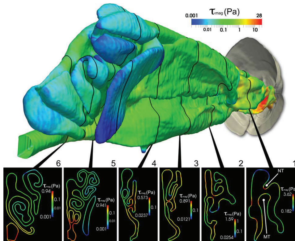
Fig. 6. Distribution of shear stress magnitude in the nasal airway of the mouse (shown in posterolateral view) from a CFD simulation of respiratory airflow in the nose. The insets show contours of shear stress magnitude ( \tau_{\text{mag}} ) on transverse cross sections of the airway wall in the respiratory (1–4) and olfactory (5,6) regions. NT, nasoturbinate; MT, maxilloturbinate. Caudal to the left, rostral to the right.
