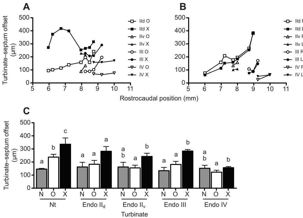
Fig. 5. Distance (offset) from medial-most border of NT and the ethmoturbinates to closest point of nasal septum. (A) Data from one UNO subject showing turbinates II–IV on occluded side are shifted laterally compared with the open side. (B) Data from one control mouse showing high degree of symmetry in turbinate offset. (C) Mean ( \pm s.e.m.) of group data pooled across rostrocaudal samples. Values with different lowercase letters are significantly different by paired or un-paired t -test ( P < 0.05 ). L, left; N, normal controls; O, open (non-occluded fossa); R, right; X, closed (occluded fossa).
