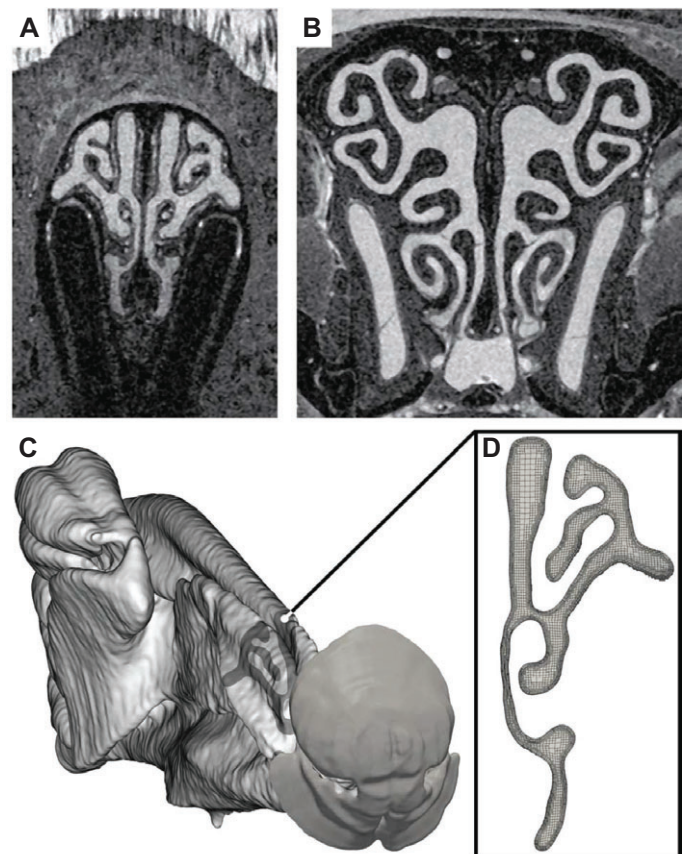
Fig. 8. Anatomically accurate computational model of the mouse nasal cavity. High-resolution MRI scans (A,B) were acquired in a cadaver specimen and were used to reconstruct a three-dimensional surface model of the right nasal airway (C). (D) A high-fidelity computational mesh of the nasal airway was generated from the anatomical reconstruction and used in computational fluid dynamics (CFD) simulations of nasal airflow.
