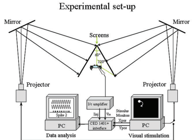
Fig. 1. The setup for visual stimulation and intracellular recording. For simplicity, one computer is shown as controlling the visual stimulus either on the right or the left screen via a switch. In practice, two computers were used, one controlling each projector (see Materials and methods for further details). I/c amplifier, intracellular amplifier; I_{inj} , current injection monitor; V_{in} , intracellular recorded membrane potential; x_{pos} , y_{pos} , x - and y -coordinates of visual stimulus, respectively.
