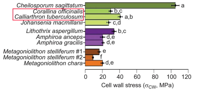
Fig. 7 (original). Cell wall material breaking stress of each species. Incorrect labels are highlighted in red.
