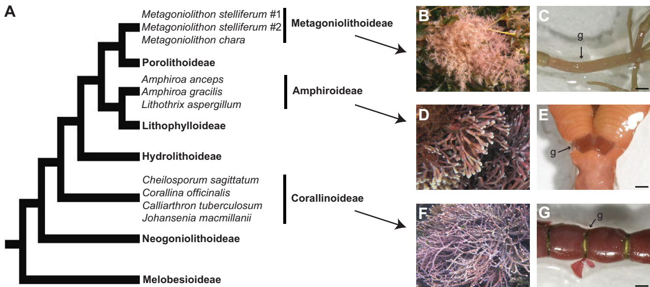
Fig. 1. Evolutionary relationships between articulated coralline subfamilies and select crustose subfamilies, showing similarities in thallus morphology and differences in genicular morphology. (A) Phylogenetic summary of relationships between coralline subfamilies (in bold) (information from Kato et al., 2011). 'Amphiroideae' refers to Amphiroideae sensu Johansen (1981), and is separated from the rest of Lithophylloideae here for clarity. (B,D,F) Coralline fronds in situ . (C,E,G) Close-up of genicula (g) under a dissecting microscope. Scale bars, 700 \mu\text{m} . (B,C) Calliarthron tuberculosum (Postels & Ruprecht) E. Y. Dawson. (D,E) Amphiroa anceps (Lamarck) Decaisne. (F,G) Metagoniolithon stelliferum #1 (Lamarck) Ducker.
