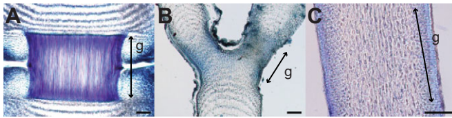
Fig. 2. Long-sections of genicula under light microscopy, dyed with 1% Aniline Blue. Scale bars, 100 \mu\text{m} . Arrows and 'g' labels indicate location of genicular tissue – note that all tissue shown in C is genicular tissue. (A) Calliarthron tuberculosum (Postels & Ruprecht) E. Y. Dawson. (B) Amphiroa gracilis Harvey. (C) Metagoniolithon stelliferum #1 (Lamarck) Ducker.
