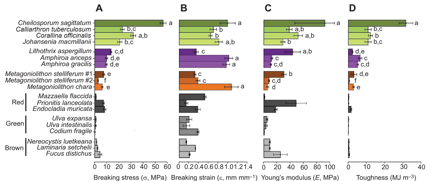
Fig. 4. Material properties of genicular tissue in tension. (A) Breaking stress, (B) breaking strain, (C) Young's modulus and (D) breaking energy of each species. Corallinoid species are in green, amphiroid species are in purple and metagoniolithoid species are in orange. Significant differences between species were found for breaking stress, breaking strain, Young's modulus and breaking energy (Kruskal–Wallis tests, P < 0.001 in all cases). Lowercase letters indicate results of a non-parametric post hoc Dunn's test ( P < 0.05 ). Grey bars show comparative data for fleshy algae: red (=Rhodophyta), brown (=Ochrophyta, Phaeophyceae) and green (=Chlorophyta) from Hale (2001). Error bars represent s.e.m.
