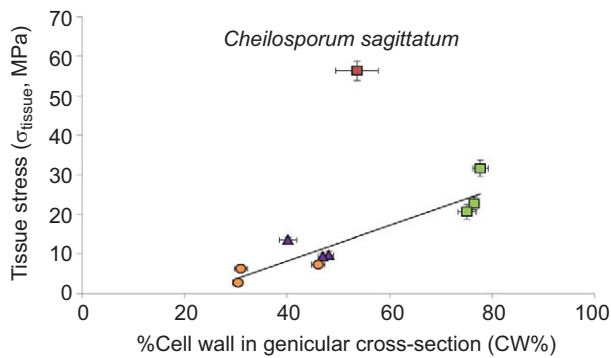
Fig. 8. Whole tissue breaking stress in genicula increases with an increase in the percentage of cross-section taken up by cell wall. Each point represents species averages. Corallinoid species (excluding Cheilosporum sagittatum ) are in green, amphiroid species are in purple and metagonioliithoid species are in orange. Cheilosporum sagittatum is shown as an outlier in red. The trend line represents the line of best fit through all points excluding C. sagittatum ( y=0.45-9.79 , R^2=0.8419 ). Error bars represent s.e.m.
