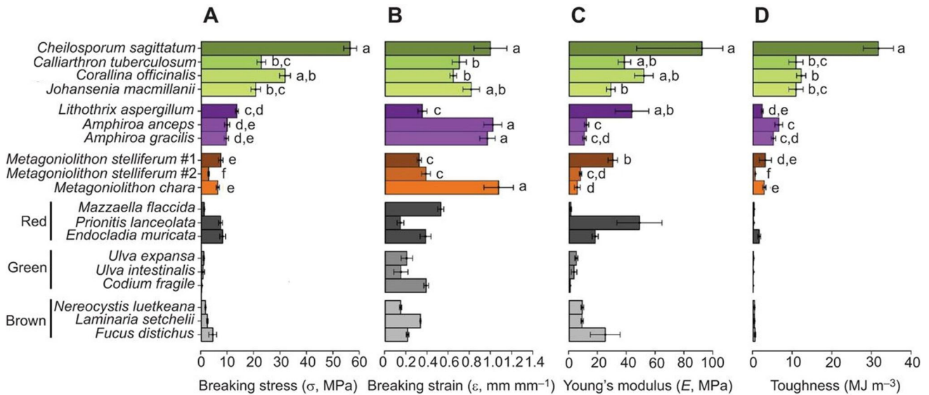
Fig. 4 (corrected). Material properties of genicular tissue in tension.
