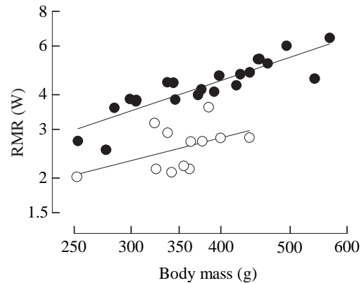
Fig. 2. Resting metabolic rate (RMR) as a function of body mass ( M_b ) in controls (filled symbols) and diet-restricted nestlings (open symbols) of European shags. The axes are log-scaled, and linear regression lines are shown for each treatment group [log RMR controls = 0.87(\pm 0.11) \times \log M_b - 1.62(\pm 0.28) , r = 0.88 ; log RMR diet-restricted = 0.66(\pm 0.37) \times \log M_b - 1.27(\pm 0.95) , r = 0.49 ].
