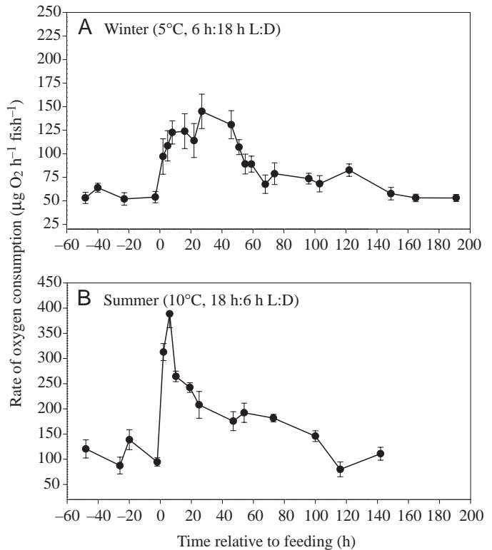
Fig. 1. Time-course of oxygen consumption following the ingestion of a single meal of amphipods in Harpagifer bispinis acclimatized to conditions of temperature and photoperiod simulating (A) winter and (B) summer. Values are means \pm S.E.M. N=6 for both groups.
