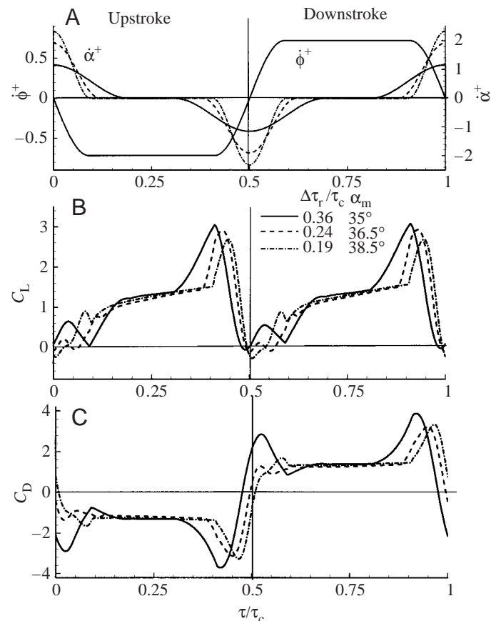
Fig. 13. Non-dimensional angular velocity of pitching rotation \alpha^+ and azimuthal rotation \phi^+ (A), lift coefficient C_L (B) and drag coefficient C_D (C) versus time during one cycle for three different values of the non-dimensional duration of wing rotation \Delta\tau_r . Symmetrical rotation; mean lift coefficient \overline{C_L}=1.15 (midstroke angle of attack \alpha_m was adjusted to make the mean lift equal to insect weight). \tau_c , non-dimensional period of one flapping cycle; \tau , non-dimensional time.
