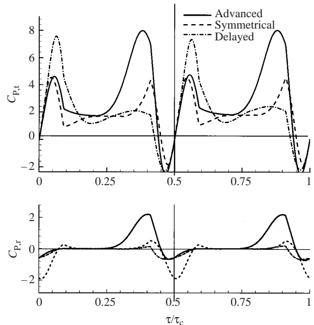
Fig. 12. The power coefficients for translation ( C_{P,t} ) and rotation ( C_{P,r} ) versus time during one cycle for the different wing rotation timings (midstroke angle of attack \alpha_m=35^\circ , non-dimensional duration of wing rotation \Delta\tau_r=0.36\tau_c ). \tau_c , non-dimensional period of one flapping cycle; \tau , non-dimensional time.
