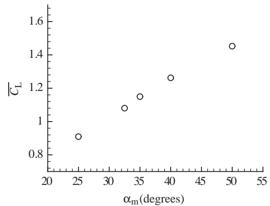
Fig. 6. Mean lift coefficient \bar{C}_L versus midstroke angle of attack \alpha_m (symmetrical rotation, non-dimensional duration of wing rotation \Delta\tau_r=0.36\tau_c , where \tau_c is the non-dimensional period of one flapping cycle).
