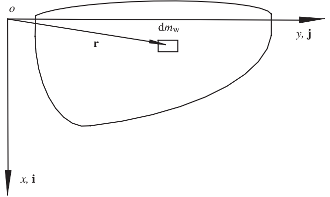
Fig. 3. Diagram showing how the moments and product of inertia are computed. o , x , y , coordinates in wing-fixed frame of reference; dm_w , mass element of the wing; \mathbf{r} , vector distance between point o and a mass element of the wing; \mathbf{i} , \mathbf{j} , unit vectors in the x and y directions, respectively.
