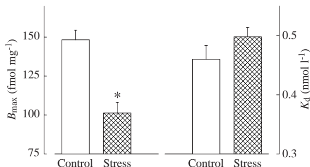
Fig. 3. Concentration ( B_{\max} , \text{fmol mg}^{-1} protein) and dissociation constant ( K_d , \text{nmol l}^{-1} ) of gill corticosteroid receptors from juvenile rainbow trout sampled 3 days after cessation of daily handling stress ( N=6 ). The fish were stressed twice daily over a period of 10 days. An asterisk indicates that the value for the stressed group was significantly different from that for the control group ( P<0.01 ). Values are means + 1 S.E.M.
