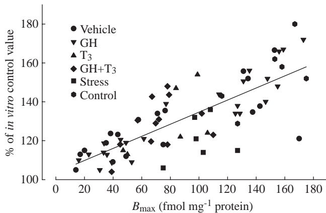
Fig. 7. In vitro Na + /K + -ATPase activity for gill filaments incubated with 10 µg ml -1 cortisol plotted against gill corticosteroid receptor concentration ( B_{\max} ). Values are in vitro gill Na + /K + -ATPase as a percentage of in vitro gill Na + /K + -ATPase activity in control filaments not treated with cortisol. Values are for fish from experiment 2 injected with vehicle (vegetable oil), 5.0 µg g -1 ovine growth hormone (GH), 1.6 µg g -1 triiodothyronine (T 3 ) or 5.0 µg g -1 GH + 1.6 µg g -1 T 3 and for fish from experiment 1 subjected to daily handling stress. Each point corresponds to one individual. The equation for the regression line is y=0.311x+103.6 ( r^2=0.614 , P=0.001 ).
