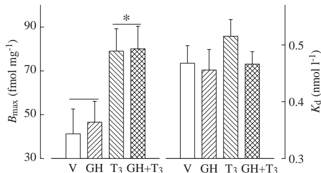
Fig. 5. Concentration ( B_{\max} , \text{fmol mg}^{-1} protein) and dissociation constant ( K_d , \text{nmol l}^{-1} ) of gill corticosteroid receptors from juvenile rainbow trout treated with vehicle (V, vegetable oil), 5.0 \mu\text{g g}^{-1} ovine growth hormone (GH), 1.6 \mu\text{g g}^{-1} triiodothyronine ( T_3 ) or 5.0 \mu\text{g g}^{-1} GH + 1.6 \mu\text{g g}^{-1} T_3 . An asterisk indicates that values for the T_3 -treated groups are significantly different from those for groups not treated with T_3 ( P<0.01 ). Values are means + 1 S.E.M., N=6 .
