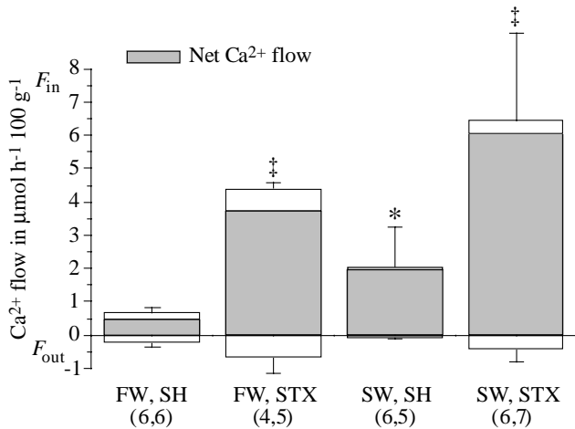
Fig. 1. Effects of stanniectomy on branchial \text{Ca}^{2+} inflow ( F_{\text{in}} ) and \text{Ca}^{2+} outflow ( F_{\text{out}} ) in eel. Calcium flows were determined with ^{45}\text{Ca} -tracer techniques in sham-operated (SH) or stanniectomised (STX) eels adapted to fresh water (FW) or to sea water (SW). Values are means \pm S.D. Numbers of fish examined are indicated in parentheses (inflow, outflow). ‡Significantly different \text{Ca}^{2+} inflow from the sham-operated group in the same medium; *significantly different \text{Ca}^{2+} inflow from the freshwater group. As there were no significant effects of salinity on \text{Ca}^{2+} outflow, the data for freshwater and seawater eels were pooled for statistical analysis. Stanniectomy yielded a 3.5-fold stimulation of \text{Ca}^{2+} outflow.
