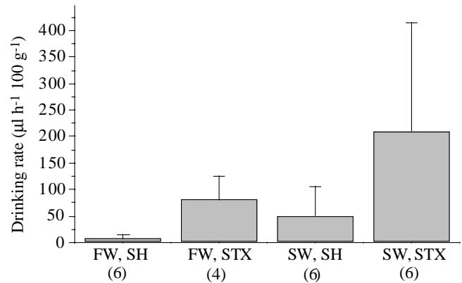
Fig. 2. Drinking rates ( \mu\text{l h}^{-1} 100 \text{ g}^{-1} ) of sham-operated (SH) and stanniectomised (STX) eels, adapted to fresh water (FW) or to sea water (SW) at 20^\circ\text{C} . Drinking rates were calculated from intestinal ^{45}\text{Ca} content after a 3 h inflow period. Values are means \pm S.D. Numbers of fish examined are in parentheses. There was no significant effect of salinity on drinking rate, and stanniectomy stimulated drinking fivefold (data from freshwater and seawater eels pooled).
