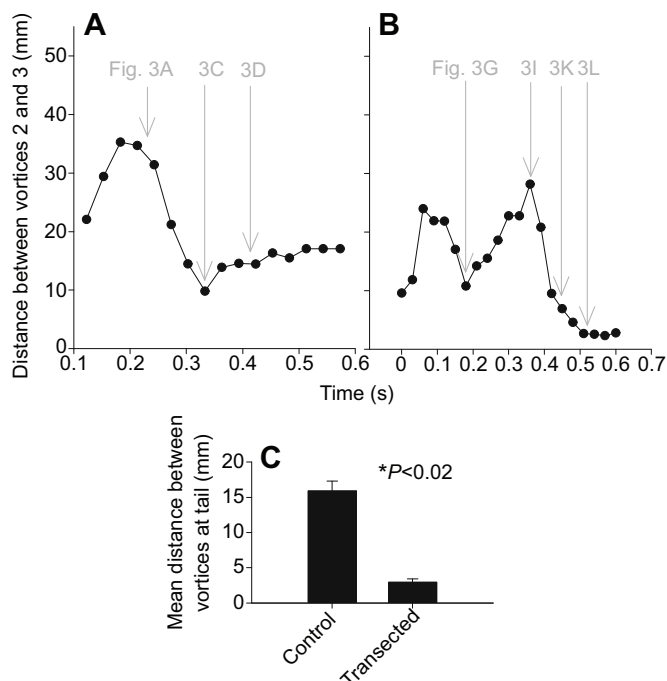
Fig. 5. Distance between adjacent vortices as they travel from the head to the tail of the control and the mid-body transected lampreys. (A) Control; (B) mid-body transected. (C) Means \pm s.d. distance between the vortices at the tail (Student's t -test, N=3 control and 2 mid-body transected). Distance was measured as the shortest distance between vorticity contours of 10 \text{ s}^{-1} .
