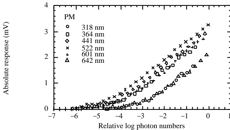
Fig. 6. Intensity curves for a PM eye in its night state when stimulated with different wavelengths.
