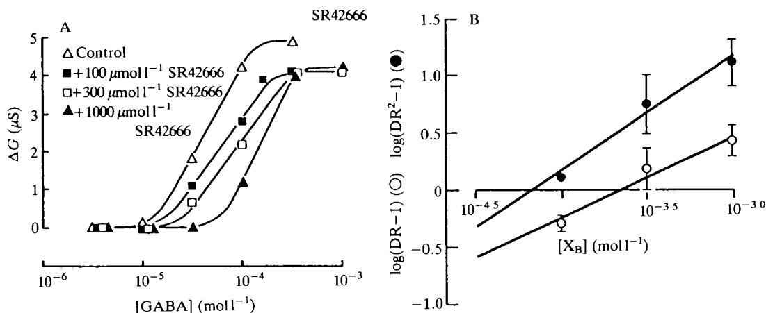
Fig. 6. Dose-dependency of the antagonism produced by SR42666. The lines correspond to the fitted modified Hill equation, whereas the points are the experimental data. (A) Dose-response curves for GABA. Control GABA dose-response curve ( \Delta ); values estimated for the modified Hill equation are \Delta G_{max}=4.9\ \mu S , EC_{50}=39.9\ \mu mol\ l^{-1} , n=2.1 . GABA dose-response curve in the presence of 100\ \mu mol\ l^{-1} SR42666 ( \blacksquare ), values estimated for the modified Hill equation are \Delta G_{max}=4.1\ \mu S , EC_{50}=59.8\ \mu mol\ l^{-1} and n=1.7 . GABA dose-response curve in the presence of 300\ \mu mol\ l^{-1} SR42666 ( \square ), values estimated for the modified Hill equation are \Delta G_{max}=4.3\ \mu S , EC_{50}=89.7\ \mu mol\ l^{-1} and n=1.8 . GABA dose-response curve in the presence of 1000\ \mu mol\ l^{-1} SR42666 ( \blacktriangle ), values estimated for the modified Hill equation are \Delta G_{max}=4.3\ \mu S , EC_{50}=134.4\ \mu mol\ l^{-1} and n=3.2 . In this particular cell \Delta G_{max} appears to be smaller in the presence of SR42666. However, in other cells, \Delta G_{max} can be higher in the presence of SR42666 than for the control. This illustrates the difficulty in measuring high membrane conductance accurately. SR42666 and the other arylaminopyridazine GABA derivatives tested quantitatively did not affect \Delta G_{max} or n significantly. (B) Schild and modified Schild plots; ( \circ ) Schild plot, \log(DR-1)/\log[X_B] , where X_B is the concentration of antagonist. Correlation coefficient, r=0.78 ; slope= 0.73\pm0.17 , P=0.001 ( F -test); R^2=0.62 . ( \bullet ) Modified Schild plot, \log(DR^2-1)/\log[X_B] . Correlation coefficient r=0.78 ; slope= 1.02\pm0.25 , P=0.001 , ( F -test); R^2=0.62 . Values are mean \pm s.e., N=13 .
