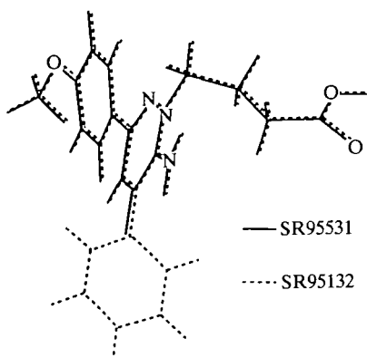
Fig. 7. Superimposition of SR95132 and SR95531. The superimposition of these two analogues shows that the 4-substituent is found in the proximity of the GABA recognition site. The inactivity of 4-substituted analogues at the vertebrate GABA A receptor was explained in terms of restriction of the free access zone required for interaction with the receptor. The volume occupied by the phenyl group of SR95132 is visualized. (Reproduced from Wermuth and Rognan, 1987, with permission.)
