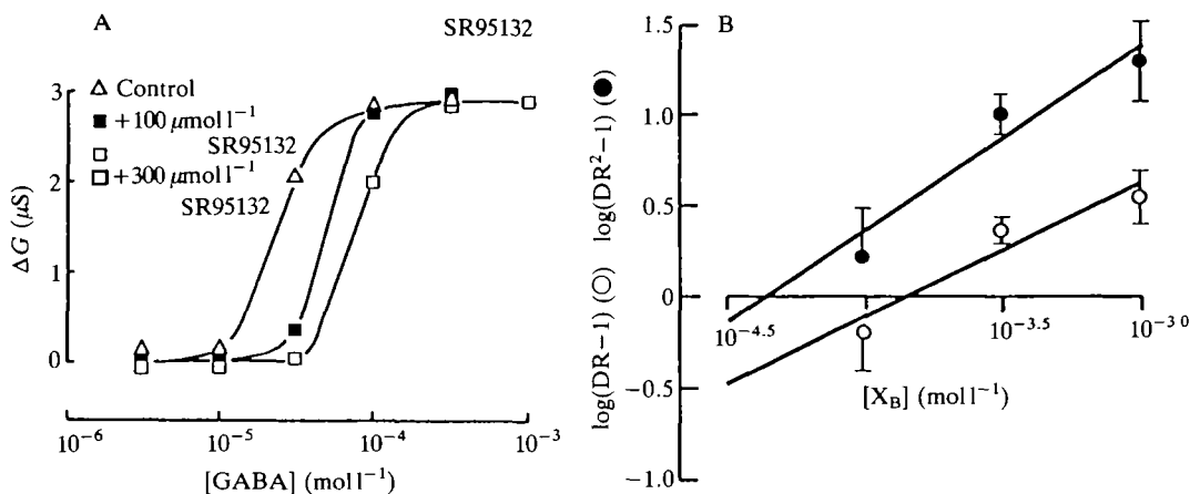
Fig. 4. Dose-dependency of the antagonism produced by SR95132. The lines correspond to the fitted modified Hill equation, whereas the points are the experimental data. (A) Dose-response curves for GABA. Control GABA dose-response curve ( \Delta ); values estimated for the modified Hill equation are \Delta G_{max}=2.8\ \mu S , EC_{50}=19.8\ \mu mol\ l^{-1} , n=2.6 . Dose-response curve for GABA in the presence of 100\ \mu mol\ l^{-1} SR95132 ( \blacksquare ), values estimated for the modified Hill equation are: \Delta G_{max}=2.8\ \mu S , EC_{50}=37.6\ \mu mol\ l^{-1} and n=3.2 . Dose-response curve for GABA in the presence of 300\ \mu mol\ l^{-1} SR95132 ( \square ), values estimated for the modified Hill equation are: \Delta G_{max}=2.8\ \mu S , EC_{50}=77.2\ \mu mol\ l^{-1} and n=3.5 . (B) Schild and modified Schild plots; ( \circ ) Schild plot, \log(DR-1)/\log[X_B] , where [X_B] is the concentration of antagonist. Correlation coefficient, r=0.71 ; slope= 0.74\pm0.25 , P=0.02 ( F -test); R^2=0.62 . ( \bullet ) Modified Schild plot, \log(DR^2-1)/\log[X_B] . Correlation coefficient r=0.75 ; slope= 1.06\pm.32 , P=0.01 , ( F -test); R^2=0.66 , suggesting a better fit than with the classical Schild plot. Values are mean \pm s.e., N=9 .
