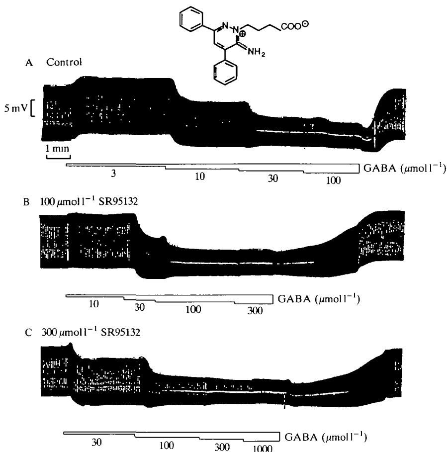
Fig. 3. Effects of 100 and 300 \mu\text{mol l}^{-1} SR95132 on the GABA dose-response relationship. (A) Control responses to cumulative application of GABA. Note the small depolarization observed with 3 \mu\text{mol l}^{-1} GABA where there was no detectable change in membrane input conductance. (B) The effect of 100 \mu\text{mol l}^{-1} SR95132. (C) The effect of 300 \mu\text{mol l}^{-1} SR95132. The corresponding dose-response curves are illustrated in Fig. 4. All three recordings were obtained from the same cell.
