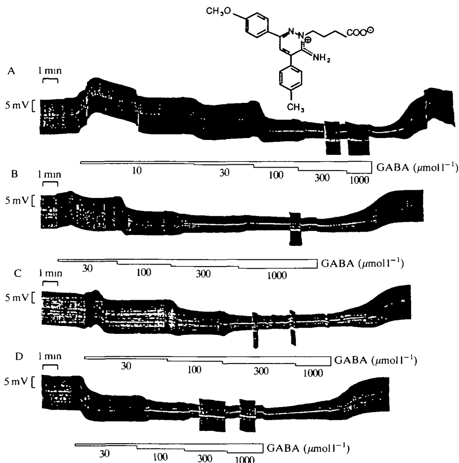
Fig. 5. Effects of 100, 300 and 1000 \mu\text{mol l}^{-1} SR42666 on the GABA dose-response relationship. (A) Control responses to cumulative application of GABA, G_0 = 2.2 \mu\text{S} . Note the transient depolarizing response in the presence of 10 \mu\text{mol l}^{-1} GABA and the temporary increase in gain from 5 mV to 2 mV per division during the application of 300 and 1000 \mu\text{mol l}^{-1} GABA. (B) In the presence of 100 \mu\text{mol l}^{-1} SR42666. Note the temporary increase in gain from 5 mV to 2 mV per division during the application of 1000 \mu\text{mol l}^{-1} GABA. (C) In the presence of 300 \mu\text{mol l}^{-1} SR42666. Note the temporary increase in gain from 5 mV to 2 mV per division during the application of 300 and 1000 \mu\text{mol l}^{-1} GABA. (D) In the presence of 1000 \mu\text{mol l}^{-1} SR42666. Note the gain changes in the presence of 300 and 1000 \mu\text{mol l}^{-1} GABA. The corresponding dose-response curves are illustrated in Fig. 6.
