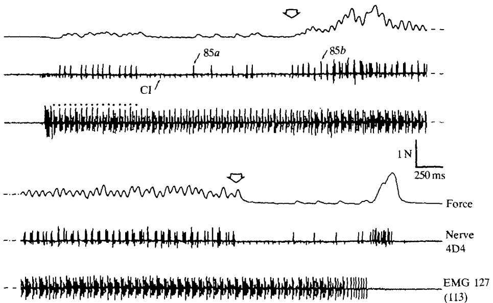
Fig. 11. Activity of motor units M85 a and M85 b . In a tethered animal with one forewing removed, pleuroalar muscle force (top trace), activity in N4D4 (middle trace) and a hindwing first basalar EMG (bottom trace; plus pick-up from M113, initial M127 potentials marked by dots for identification) were recorded. The smallest spikes in the neurogram are from CI 1 . Unit a produced the middle-sized action potentials, unit b the largest ones. The animal flew undisturbed at the beginning and end of the sequence. Arrows mark start and termination of a visual roll stimulus.
