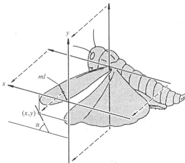
Fig. 2. Evaluation of photogrammetry experiments. Photographic exposures (camera centred on forewing hinge, perpendicular to the animal's sagittal plane) represent parallel projections of the wing movement onto the film plane (dashed lines). The image of the wing hinge was taken as the origin of the coordinate system for evaluation (abscissa horizontal) and the image of the marker line ( ml ) on the forewing was evaluated. Centre coordinates ( x,y ) and supination angle \alpha of the line's image were determined for computer-aided calculation of the angular setting of the wing.
