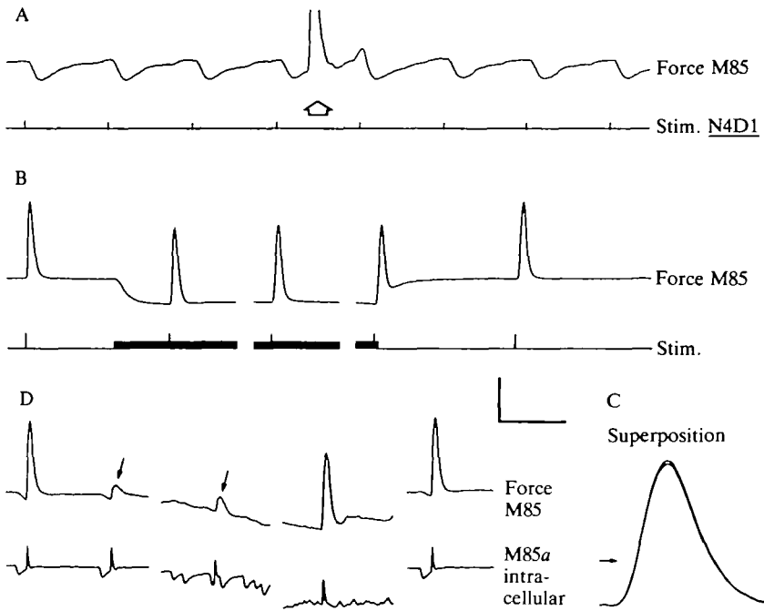
Fig. 7. CI activity reduces basic tonus. (A) Mesothoracic CI_1 was stimulated (in N4D1, bottom trace) and the force output of M85 recorded (top trace). Each stimulus, i.e. spike of CI, caused a transient relaxation of M85 (see also Fig. 6A). The effect persisted after transection of N4 root (arrow and movement artefact in the middle). (B) Both excitors of M85 were stimulated in N4D4 (stimulus frequency about 1 Hz, bottom trace), CI_1 was activated in N3A3 (stimulus frequency 50 Hz, black bar in bottom trace) and M85 force output was recorded (top trace). CI stimulation reduced basic tonus but left muscle twitches almost unaffected. (C, inset) One muscle twitch elicited with simultaneous CI stimulation (smaller twitch) and one without (larger twitch) are superimposed to demonstrate the minute effect of CI activity on twitch amplitude (approx. 2% decrease; time scale 10 times, amplitude two times expanded, arrow indicates level of basic tonus without CI stimulation). (D) During the experiment described in Fig. 6 spontaneous struggling of the animal occurred, accompanied by strong CI_1 discharges (two middle segments, IJP rate 25–35 Hz). Reductions in membrane potential and basic tonus and constancy of EJPs and twitch responses are visible. Recordings from the quiescent animal are presented in the first and last segment, only unit a was activated in the second and third muscle twitch shown (arrows). Scale bars, 500 ms, 0.1 mN in A, 0.3 mN in B; 400 ms, 35 mV or 0.25 mN in D.
