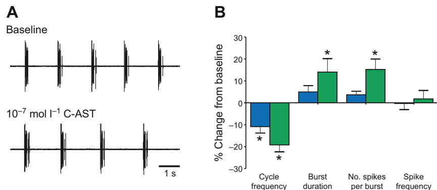
Fig. 9. C-AST decreased cycle frequency but had mixed effects on burst parameters in the isolated CG. (A) CG neuronal output was recorded extracellularly from a motor nerve. (B) Data from lobsters were analyzed according to their response to 10^{-7} mol l ^{-1} C-AST (increase in contraction amplitude, green bars, N=16 ; decrease in contraction amplitude, blue bars, N=15 ) in the semi-intact heart preparation before the CG was removed for recording. Superfusion of 10^{-7} mol l ^{-1} C-AST over the isolated CG caused a decrease in burst cycle frequency in all preparations; means for the two groups did not differ significantly. There was a clear increase in burst duration and number of spikes per burst only among lobsters in which the peptide increased contraction amplitude in the semi-intact heart, while no effect on these two parameters was observed in lobsters with decreased contraction amplitude. Spike frequency did not change in either group of lobsters. * P<0.05 , t -test. Error bars show s.e.m.
