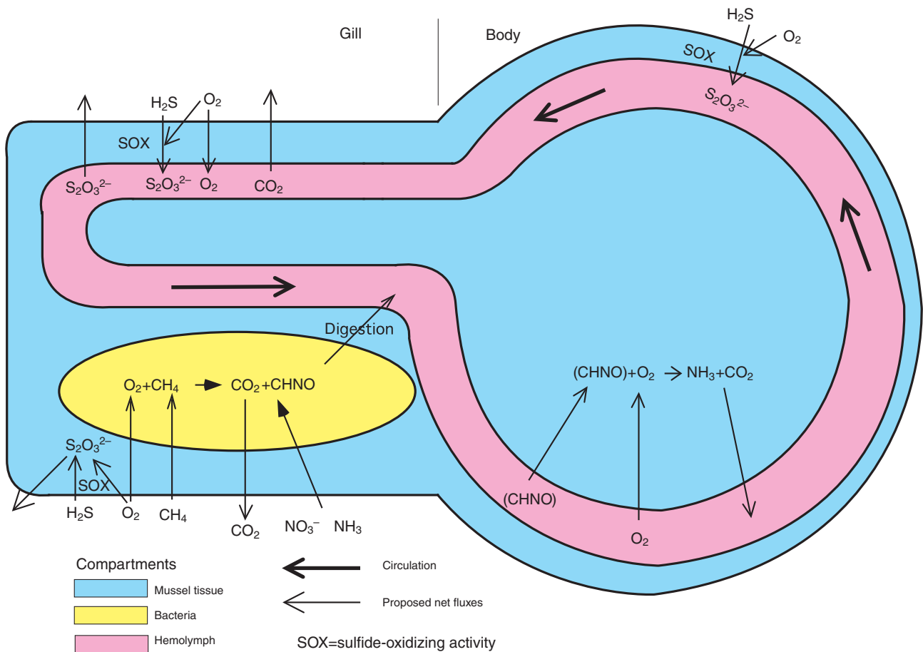
Fig. 5. A schematic diagram of the physiological functioning of a mussel with methane-oxidizing symbionts, such as Bathymodilus childressi . Light blue represents animal tissue. Yellow represents the endosymbiotic bacteria. Pink represents the vascular fluid. The bold arrows represent vascular fluid flow. The thin arrows represent diffusion, chemical reactions or chemical equilibration depending on the context. SOX indicates the presence of a sulfide-oxidizing activity which oxidizes sulfide to thiosulfate. 'Digestion' indicates that the symbionts are digested within the bacteriocytes in the gills. CHNO indicates organic matter from the digested bacteria. Because of substantial environmental sulfide concentrations, sulfide oxidation by the animal is required for control of the toxicity of sulfide within symbiosis even though sulfide is not utilized by the symbionts.
