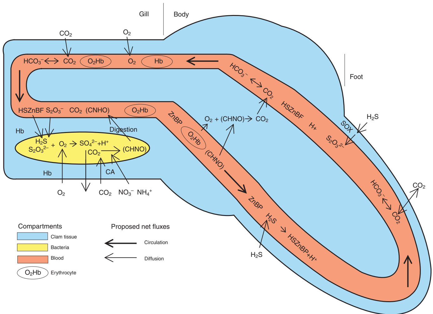
Fig. 3. A schematic diagram of the physiological functioning of the vesicomyid clam Calyptogena magnifica . Light blue represents animal tissue. Yellow represents the endosymbiotic bacteria. Orange represents the vascular fluid. Pink represents the coelomic fluid. The bold arrows represent blood flow. The thin arrows represent diffusion, chemical reactions or chemical equilibration depending on the context. Thin arrows crossing tissue boundaries are diffusion or unknown transport mechanisms. Hb represents hemoglobin and it is contained in erythrocytes depicted as ovals within the vascular fluid. BP indicates a separate protein, found in the vascular fluid, which binds sulfide to a site incorporating zinc. CA indicates carbonic anhydrase. SOX indicates the presence of a sulfide-oxidizing activity which oxidizes sulfide to thiosulfate. 'Digestion' indicates that the symbionts are digested within the bacteriocytes in the gills. CHNO indicates organic matter from the digested bacteria. The dominant uptake route for sulfide is believed to be across the foot, which is extended into the substrate, while the other metabolites are taken up across the gills. This schematic diagram is applicable to all members of the family Vesicomyidae. Figure adapted from Childress and Fisher (Childress and Fisher, 1992).
