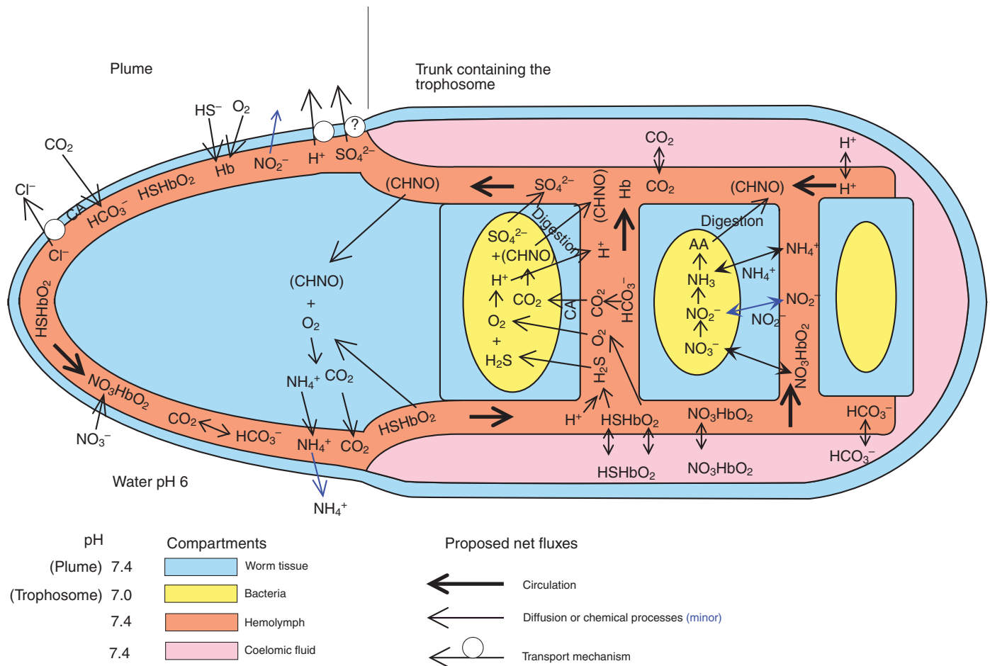
Fig. 2. A schematic diagram of the physiological functioning of the hot vent siboglinid tubeworm Riftia pachyptila . Light blue represents worm tissue with an intracellular pH of 7.4 (Goffredi et al., 1999a). Yellow represents the endosymbiotic bacteria (intracellular pH of trophosome bacteria and bacteriocytes is 7.0). Orange represents the vascular fluid with a strongly defended pH of 7.4. Pink represents the coelomic fluid with a pH near 7.4 but slightly above the hemolymph pH. The bold arrows represent blood flow. The thin arrows represent diffusion, chemical reactions or chemical equilibration depending on the context. Thin arrows crossing tissue boundaries are diffusion. (The thin blue arrows represent minor fluxes of ammonium and nitrite ions.) A thin arrow with an open circle attached represents some sort of specific transport mechanism. Hb indicates hemoglobin and it is shown as binding and carrying sulfide, oxygen and nitrate. ‘Digest’ indicates that the symbionts are digested within the bacteriocytes in the gills. CHNO indicates organic matter from the digested bacteria. AA indicates amino acids. Nitrogen metabolism is separated from sulfide and carbon metabolism just for convenience in depiction. All other chemical labels have their usually accepted meanings. This schematic diagram is representative of the functioning of the Eastern Pacific hot vent tubeworms Riftia pachyptila , Oasisia alvinae , Tevnia jerichonana and Ridgeia piscesae . As discussed in the text, the cold seep tubeworms have essentially the same physiological system except that the uptake of sulfide is through extensions of the posterior of the body deep into sulfide-rich sediments. Figure adapted from Childress and Fisher (Childress and Fisher, 1992).
