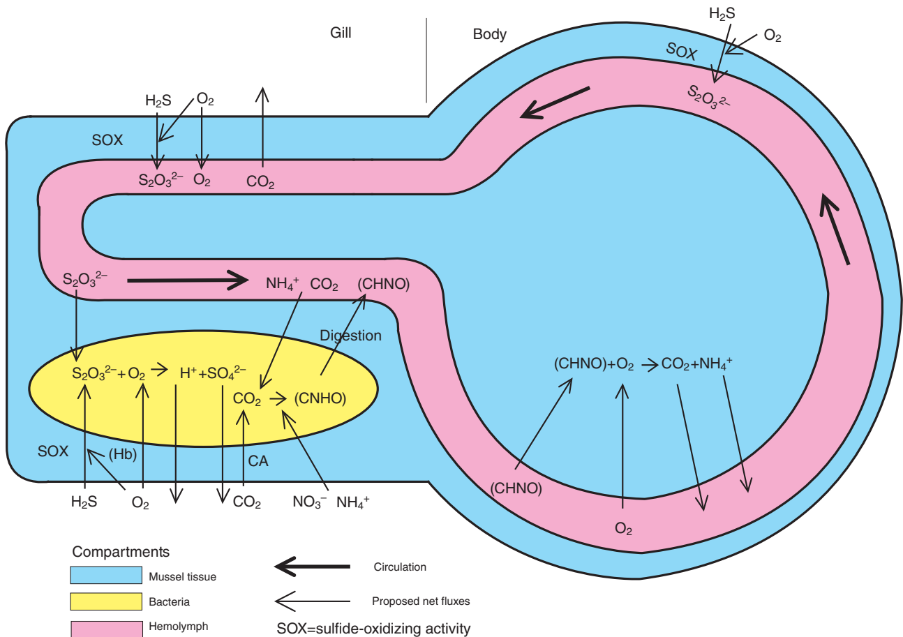
Fig. 4. A schematic diagram of the physiological functioning of a mussel with sulfide-oxidizing symbionts, such as Bathymodilus thermophilus . With certain modifications described below this is applicable to all of the molluscan endosymbioses except the Vesicomyidae. Light blue represents animal tissue. Yellow represents the endosymbiotic bacteria. Pink represents the vascular fluid. The bold arrows represent vascular fluid flow. The thin arrows represent diffusion, chemical reactions or chemical equilibration depending on the context. Thin arrows crossing tissue boundaries are diffusion or unknown transport mechanisms. CA indicates carbonic anhydrase. SOX indicates the presence of a sulfide-oxidizing activity which oxidizes sulfide to thiosulfate. 'Digestion' indicates that the symbionts are digested within the bacteriocytes in the gills. CHNO indicates organic matter from the digested bacteria. All other molluscan endosymbioses, bivalves and gastropods have gill hemoglobins [shown as (Hb)], often in high concentrations, which are very likely to be important in the uptake and sequestering of sulfide and oxygen in these symbioses. In addition, both solemyid bivalves and provannid gastropods have substantial hemocyanin concentrations in their vascular fluids to supply the oxygen needed by the animal tissues. Further, the solemyids, unlike all the other molluscan endosymbioses studied in detail, appear to rapidly transfer a large fraction of the chemosynthate via leakage from the bacteria instead of transferring it much more slowly after digestion of the bacteria as shown. Figure adapted from Childress and Fisher (Childress and Fisher, 1992).
