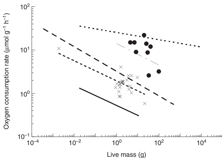
Fig. 1. The oxygen consumption rates from Table 1 of the chemoautotrophic endosymbioses (filled circles), standardized to 20^\circ\text{C} using a Q_{10} of 2, plotted with oxygen consumption rates of a variety of non-symbiotic invertebrates and fishes measured at or standardized to 20^\circ\text{C} as above. Each of the filled circles represents one species using data from Table 1. Reading from the bottom of the graph, the solid line represents data for medusae (Thuesen and Childress, 1994). The crosses (x) and short dashed line represent data from Anthopleura elegantissima (Towanda, 2008), Metridium senile (Sassaman and Mangum, 1972), Ceriatheopsis americanus (Sassaman and Mangum, 1974) and Haliplanella luciae (Zamer and Mangum, 1979). The medium dashed line represents the 'invertebrate' data including annelids, bivalves, gastropods, crustaceans and echinoderms used by Gillooly and colleagues (Gillooly et al., 2001). The long dashed line represents data on routine metabolism of horse mackerel, Trachurus trachurus (Herrmann and Enders, 2000). The line at the top with very short dashes represents routine metabolism data for loliginid and ommastrephid cephalopods (Seibel, 2007). All consumption rates are expressed relative to the live mass of the animals.
