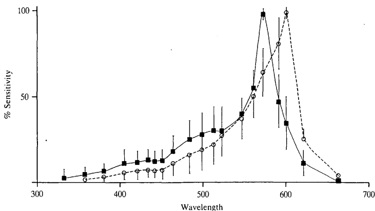
Fig. 1. Dark-adapted (DA) spectral sensitivity curves. Solid line, night; broken line, day. Error bars show standard deviation, N = 12 .
