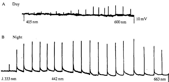
Fig. 2. Intracellularly recorded responses to monochromatic light flashes ranging from 333 nm to 663 nm. (A) Dark-adapted, day; (B) dark-adapted, night.
