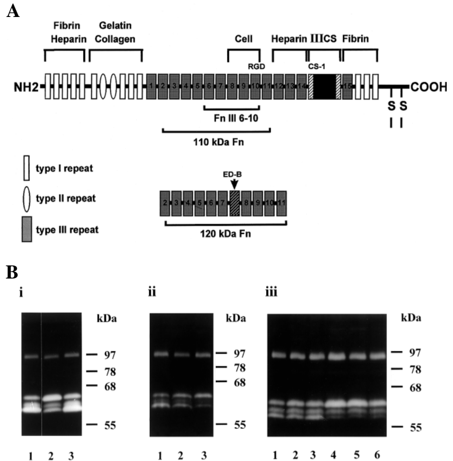
Fig. 2. Processing of proMMP-2 to the active form is up-regulated by fragments of fibronectin comprising the \alpha 5\beta 1 integrin binding site and by a monoclonal antibody to \alpha 5 integrin. (A) Schematic diagram of intact plasma fibronectin and the fibronectin fragments used in this study. (B) HT1080 cells were cultured under serum free conditions for 48 hours on fibronectin or fibronectin fragments, or on immobilised antibodies to integrin subunits. Samples of conditioned media were analysed for gelatin degrading activity by zymography. (i) Cells were cultured on fibronectin (lane 1), on laminin-1 (lane 2) or on the 120 kDa fragment (lane 3). (ii) Cells were cultured on fibronectin (lane 1), on Fn III 6-10 (lane 2) or on laminin-1 (lane 3). (iii) Monoclonal antibodies to integrin subunits were used as substrates. Cells cultured on fibronectin (lane 1), on the anti- \alpha 5 antibody mAb 16 (lane 2), on anti- \beta 1 antibody mAb 13 (lane 3), on anti- \alpha 5 antibody mAb 11 (lane 4), or on anti- \alpha 6 antibody GoH3 (lane 5). Cells cultured on laminin-1 (lane 6). Molecular mass markers are indicated on the right.
