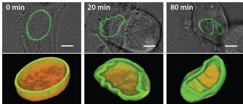
Fig. 3. Wrinkling of the nucleus envelope in a HFF cell treated with trypsin. The nuclear volume shrank by 38%. Scale bars: 5 \mu\text{m} .
