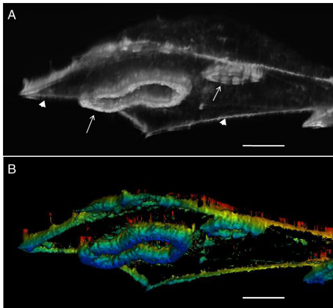
Fig. 3. Three-dimensional (3D) reconstruction of F-actin structure in a BHK-RSV cell. (A) A 3D reconstruction was derived by combining images from confocal planes viewed from the side of the basal (adherent) face. F-actin staining was carried out after fixation in 4% paraformaldehyde with TRITC-phalloidin. 3D reconstruction and rendering of the actin cytoskeleton was carried out through EDIT3D software, using grey-level images of each confocal z-stack (developed by Yves Usson and Franck Parazza, UMR CNRS 5525, Grenoble, France). Actin stress fibers are indicated by arrowheads, and the collective organization of podosomes and invadopodia by arrows. (B) A color scale was added, purely to indicate the relative position of the z-plane. The most basal plane was colored blue. Scale bars: 5 \mu m.
