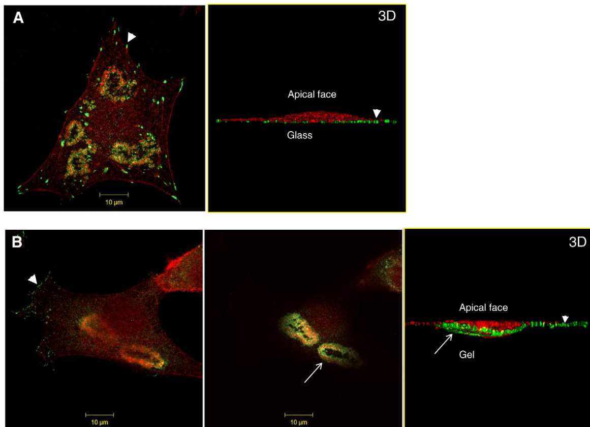
Fig. 5. Visualization of actin structure and paxillin in mRFP-actin-transfected BHK-RSV cells. (A,B) Rigid (A) and flexible (B) substrates were coated with vitronectin. Staining for paxillin (green) was carried out after fixation in 4% paraformaldehyde with anti-paxillin antibodies. 3D reconstruction (right-most images) was carried out using EDIT3D software as in Fig. 3. (A) On the left is an image from a single confocal plane of a BHK-RSV cell adherent on glass (rigid) substrate. The right image shows a 3D reconstruction. Arrowheads indicate focal adhesions. (B) Left and middle panels show images from two confocal planes of a BHK-RSV cell adherent on hydrogel made of polyacrylamide (flexible) substrate. Confocal planes were from the top of the gel (left) and inside the gel (middle). Note that focal adhesions (arrowheads) are smaller in size on the flexible substrate (B) than on the rigid one (A). (B) The 3D reconstruction (right) shows that collective organizations of podosomes or invadopodia (arrow) seem to 'push' the gel, hauling the whole cell body.
