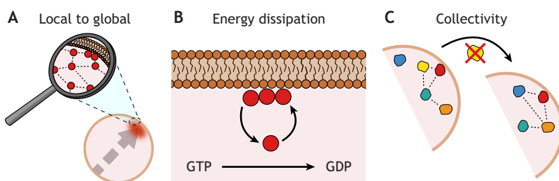
Fig. 2. Properties of self-organized structures. (A) The global ordered patterns of self-organized structures have their origin in local microscopic interactions, as opposed to an external template at the macroscopic level. (B) In contrast to self-assembly, self-organization requires energy dissipation to maintain the ordered structure, for instance through the GTPase cycle present in many polarity systems. (C) Components of self-organized structures behave as a collective: perturbing one element of the structure is likely to change the relations between other elements as well.
