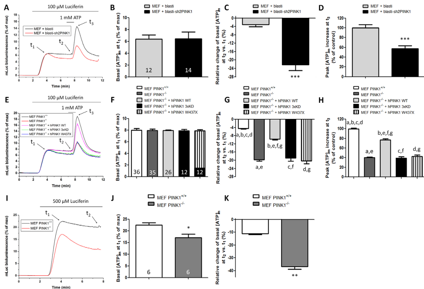
Fig. 4. Mitochondrial ATP synthesis is reduced in PINK1-deficient MEFs. Basal- and ATP-evoked increase of [ATP] M in MEFs expressing mTLUC and perfused with 100 \mu M or 500 \mu M D-luciferin. (A) [ATP] M measurements in control and PINK1-KD MEFs. (B) basal [ATP] M levels at time point t_1 , (C) relative change of basal [ATP] M values at time point t_2 , and (D) ATP-stimulated peak increase in [ATP] M (at time point t_3 ). (E–H) Luminometric analysis of [ATP] M in PINK1 wild-type and PINK1-KO MEFs, including PINK1-KO MEFs stably overexpressing human WT PINK1 or one of its mutants (3x kinase-dead and W437X). Columns labeled with the same letters show significant differences between the two conditions. (I) [ATP] M measurements in PINK1 wild-type and PINK1-KO MEFs perfused with 500 \mu M D-luciferin. Quantification of bioluminescence shows a lower basal [ATP] M level at time point t_1 (J) and a higher basal [ATP] M decrease at time point t_2 (K) in PINK1-KO MEFs compared with control cells. Number of coverslips examined is indicated on the columns. * P <0.05, ** P <0.01 and *** P <0.001 vs control group.
