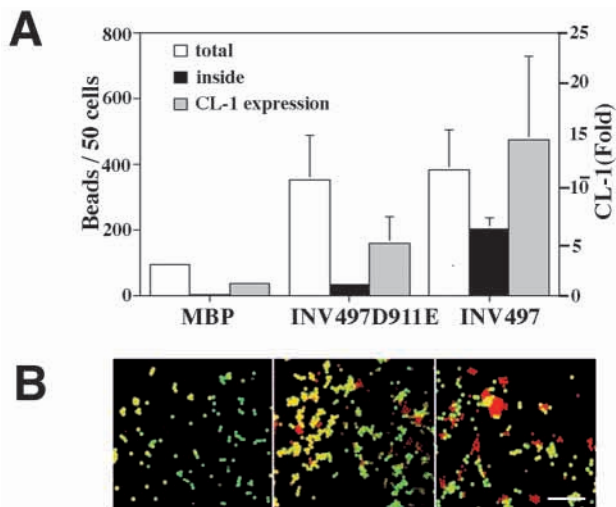
Fig. 2. Effect of affinity of invasin binding on bead phagocytosis and CL-1 induction. RSF were incubated for 2 or 24 hours with beads coated with MBP (nonspecific binding control), INV497D911E (low-affinity binding) or INV497 (high-affinity binding). Bead phagocytosis was analyzed after 3 hours and CL-1 expression was measured in the supernatant by slot blot after 24 hours. (A) Quantitative representation of bead binding and uptake after 3 hours and CL-1 expression after 24 hours for each type of coating. (B) Micrographs of the phagocytosis assay. The green beads are outside and the red beads are inside the cells. Error bars represent \pm s.e.m. of 3 independent experiments. Bar, 50 \mu m.
