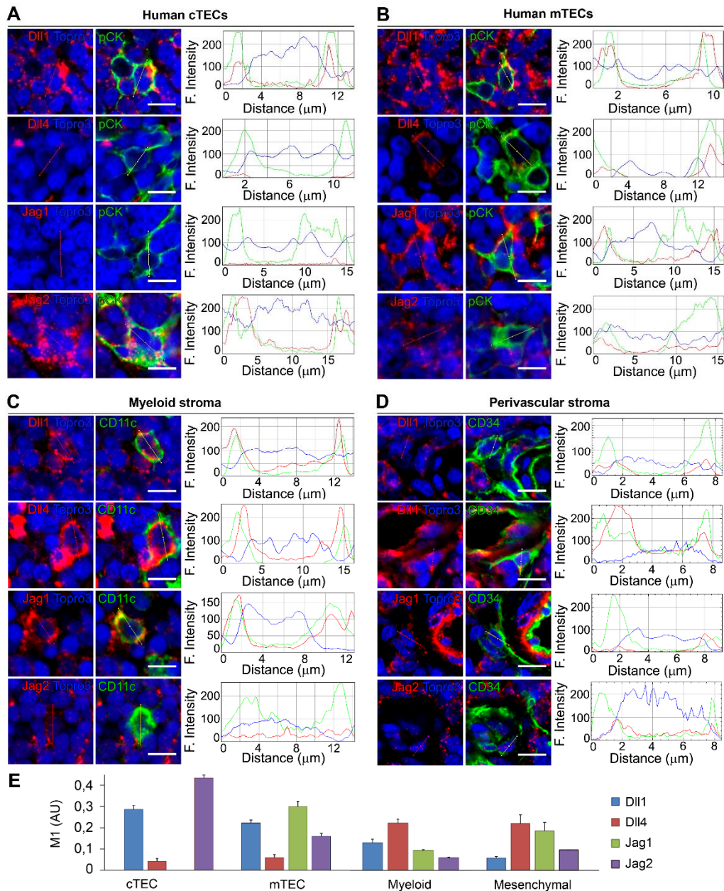
Figure S1. Co-localization analyses of Notch ligands with stromal cells in the human postnatal thymus. (A-D) Image ROIs (30μm) of postnatal human thymus sections labelled with anti-Notch ligand antibodies showing single stromal cells, including cTECs (A), mTECs (B), CD11c + (C) and CD34 + (D) and its corresponding RGB colocalization profile. RGB mean fluorescence intensity (MFI) of single stromal cells was measured by tracing a linear ROI (yellow line) along the cells. Images are representative of results obtained from at least 3 different tissue samples per ligand and stromal marker. Scale bars: 10μm. (E) Graph bars show M1 co-localization of Mander's coefficient. ICA plugin (Li et al., 2004) was applied to at least 10 images of cortical and medullary areas for each stromal marker and Notch ligand, obtained from different tissue samples (n=3).
