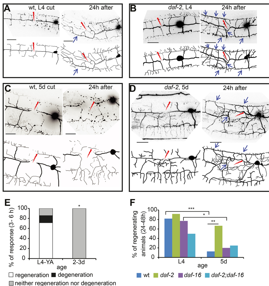
Fig. 6. daf-2(-) restores regenerative ability of aged animals via daf-16 . (A-D) Negative fluorescence images of PVD neurons immediately after cut and 24 h later in wild type (wt) and daf-2 mutants at L4 and 5d, as indicated. Below are schematics of images. Red lightning indicates injury sites; blue arrows, fusion sites (successful regeneration). Scale bars: 20 \mu m. (E) Response to injury of wild types at L4-young adult (YA) and 2-3d within a short time (3-6 h) after injury. Number of animals: L4-YA, n=7 ; 2-3d, n=4 . (F) Percentage of successfully regenerating animals within 24-48 h of injury. * P<0.05 , ** P<0.01 , *** P<0.001 (Fisher's exact tests). Number of animals analyzed: wt L4, n=22 ; wt 5d, n=16 ; daf-2 L4, n=24 ; daf-2 5d, n=12 ; daf-16 L4, n=13 ; daf-16 5d, n=10 ; daf-2 ; daf-16 L4, n=8 ; daf-2 ; daf-16 5d, n=8 . See also Movies 2-4.
