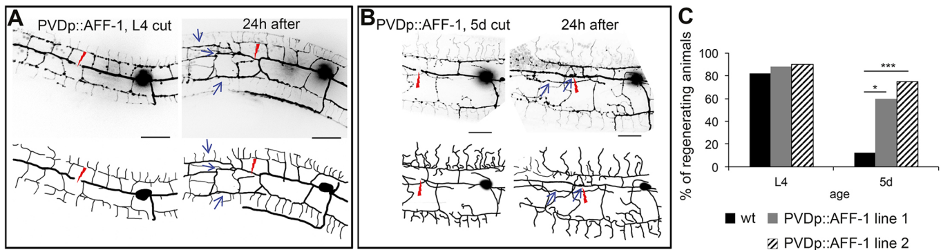
Fig. 7. AFF-1 enhances regeneration by dendrite fusion in 5d animals. (A,B) Inverted fluorescence images of PVD neurons immediately after cut and 24 h later in animals overexpressing AFF-1 in the PVD (PVDp::AFF-1), at L4 and at 5d, as indicated on each image (schematics below each image). Red lightning marks the injury site and blue arrows point to dendrite fusion sites. Scale bars: 20 \mu m. (C) Percentage of successfully regenerating animals within 24–48 h of injury. * P < 0.05 ; *** P < 0.001 (Fisher's exact test). Number of animals analyzed: wt L4, n = 22 ; wt 5d, n = 16 ; PVDp::AFF-1 line 1 L4, n = 17 ; PVDp::AFF-1 line 1 5d, n = 10 ; PVDp::AFF-1 line 2 L4, n = 15 ; PVDp::AFF-1 line 2 5d, n = 11 . See also Movies 5, 6. PVDp::AFF-1 line 1 and 2 correspond to worms carrying the extrachromosomal arrays hyEx39 and hyEx391 , respectively.
