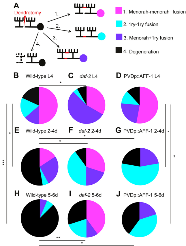
Fig. 8. daf-2(-) and AFF-1-overexpressing animals rejuvenate fusion potential of broken dendrites. (A) Schematic representing four possible outcomes of dendrotomy. Dendrite auto-fusion indicates successful regeneration (outcomes 1-3); if fusion does not occur degeneration takes place (outcome 4). (B-J) Percentages of wild-type worms, daf-2 mutants and AFF-1-overexpressing animals (PVDp::AFF-1) at different ages, divided into the four different types of response to injury as described in A. Genotype and age are listed above each plot. * P < 0.05 , ** P < 0.01 , *** P < 0.001 (Fisher's exact tests). Significant differences were also found between C and F, between C and I and between B and J ( P < 0.05 ).
