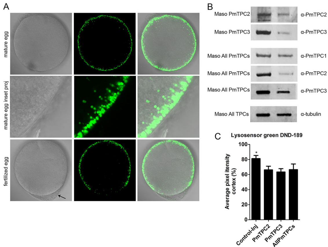
Fig. 6. PmTPC knockdown leads to increased pH in the cortical granules. (A) A mature egg labeled with lysosensor green DND-189 (upper panel). Projection of an inset in the egg cortex showing the cortical granules labeled with Lysosensor (middle panel). Labeled eggs were fertilized and the loss of Lysosensor accumulation in the regions where the cortical granules fused to form the envelope (arrow) illustrates the specificity of the Lysosensor labeling to the cortical granules (lower panels). (B) Immunoblotting showing the knockdown of PmTPCs after morpholino injections. (C) Lysosensor Green DND-189 fluorescence intensity of the egg cortex was measured using Metamorph. * P < 0.05 , one-way ANOVA.
