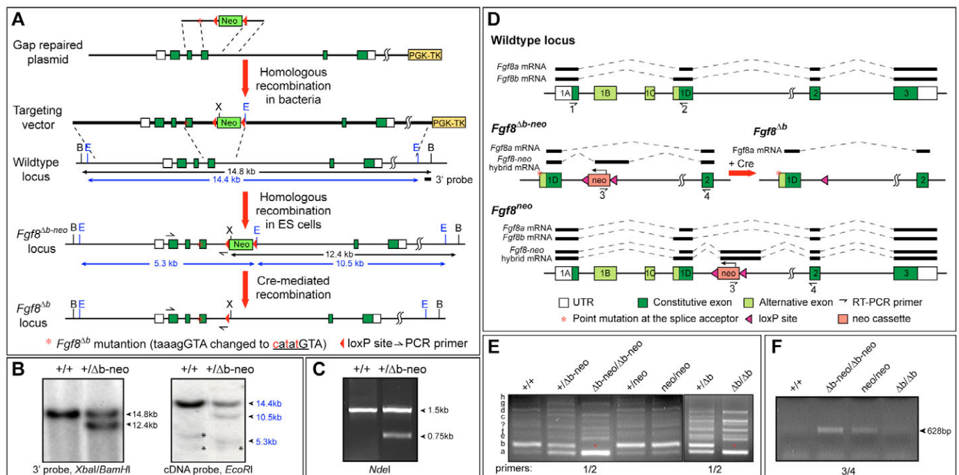
Fig. 1. Generation of splice site mutation to abolish Fgf8b expression in mouse. (A) Schematic representation of mutations in the Fgf8 locus. The change of sequences (bottom; mutations are shown in red) at the junction of intron (lowercase letters) and exon (capital letters) mutates the 5' alternative splice acceptor and creates an NdeI site (underlined). (B) Southern blot analysis to identify targeted embryonic stem (ES) cell clones. Asterisks indicate non-specific signals. (C) PCR and restriction digestion analysis to verify the point mutation. (D) Schematic representation of Fgf8 (top), Fgf8 Δb-neo (middle, left), Fgf8 Δb (middle, right) and Fgf8 neo (bottom) loci, and alterations in RNA splicing due to the point mutation and neo insertion. The Fgf8-neo hybrid transcript results from a cryptic splice donor and acceptor in the neo gene and in the intronic region 360 bp downstream to the neo gene, respectively. (E) Reverse transcriptase (RT)-PCR analysis of different Fgf8 splice variants in E7.5 embryos of indicated genotypes using primers 1 and 2 (shown in E). Fgf8 splice variants (a-h and unknown) are marked to the left. Notice that Fgf8b (asterisk) is missing in Fgf8 Δb-neo/Δb-neo and Fgf8 Δb/Δb embryos, whereas the neo insertion has no effect on the alternative splicing of the first four exons. (F) RT-PCR assay using primers 3 and 4 (indicated in D) reveals that the insertion of neo results in the production of Fgf8-neo hybrid transcripts. B, Bam HI; E, Eco RI; X, Xba I.
