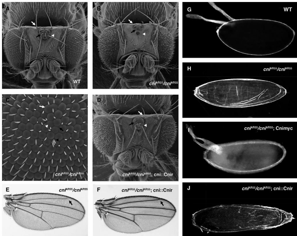
Fig. 1. cni -related and cni show partial redundancy in the soma but not the germline. (A) Wild-type head. Ocellar (arrowhead), intercellular (black arrow), and post-vertical bristles (white arrow) are marked. (B) cni AR55 / cni AR55 head. Ocellar (arrowhead), intercellular (black arrow) and post-vertical bristles (white arrow) are missing and the eyes are rough. (C) cni AR55 / cni AR55 rough eye phenotype with fusion of ommatidia (white arrow), specification of ommatidia with aberrant numbers of cone cells (white arrowhead), and missing (black arrow) or ectopic (black arrowhead) interommatidial bristles. (D) The pcni::Cnir transgene ( cnir ORF under cni control) rescues ocellar (arrowhead) and post-vertical (white arrow), but not intraocellar bristles (black arrow) or the rough eye phenotype. (E) Homozygous cni AR55 / cni AR55 wing. Vein 2 is truncated before it reaches the margin (arrow). (F) One copy of the pcni::Cnir transgene suppresses the cni wing phenotype (arrow). (G) Wild-type egg with two large dorsal respiratory appendages and an anterior micropyle. (H) Egg from a cni AR55 / cni AR55 mother. Owing to the loss of Grk signalling, the egg is ventralized and both ends differentiate into anterior structures. (I) Egg from a cni AR55 / cni AR55 female carrying a pCnimyc transgene. Establishment of the anteroposterior axis is completely rescued and that of the dorsoventral axis largely rescued. (J) Egg from a cni AR55 / cni AR55 ; pcni::Cnir female. Expression of cnir under control of cni promoter and UTR sequences fails to rescue Grk signalling.
