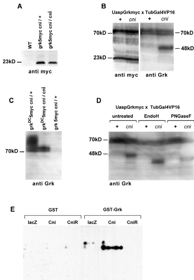
Fig. 6. Western blots with epitope tagged Grk protein and GST pull-downs. (A) Grk tagged C-terminally with five myc tags (Grk5myc) under endogenous control. Only the C-terminal cleavage residue but not a full-length precursor can be detected using the 9E10 anti-myc monoclonal. No differences are visible between homozygous cni AR55 mutant ovaries and heterozygous sibling controls. (B) Grk5myc overexpressed in wild-type (+) and homozygous cni AR55 ( cni ) ovaries using the TubGal4VP16 driver. The 9E10 anti-myc monoclonal reveals two bands. Although the lower band corresponds in size to the expected C-terminal cleavage residue, the upper band, corresponding to an uncleaved precursor, is larger than predicted from the protein sequence, indicative of glycosylation. In addition to the precursor band, the 1D12 anti-Grk monoclonal reveals a shorter band corresponding in size to the released N-terminal growth factor fragment in the mutant but not the wild-type lane. (C) A protein species corresponding in size to the uncleaved Grk precursor accumulates in lysates expressing a Grk5myc construct carrying the grk DC point mutation from the endogenous promoter (GrkDC5myc). This does not occur in ovaries expressing the functional Grk5myc version. Smearing of the GrkDC5myc band into several high molecular weight species indicative of Golgi glycosylation only occurs in the presence of Cni. (D) The N-terminal growth factor fragment accumulating in cni mutant ovaries upon Grk overexpression is sensitive to EndoH and PNGaseF, indicating ER-type high Mannose glycosylation. (E) Grk and Cni interact directly. MBP fusion proteins with lacZ or the N-terminal 57 amino acids of Cni or CniR were pulled down using GST or GST-Grk (GST fused to Grk amino acids 179-245) prebound to beads. Probing the pellets with anti-MBP antibody reveals a specific interaction between the juxtamembrane domain of Grk and the Cni N terminus.
