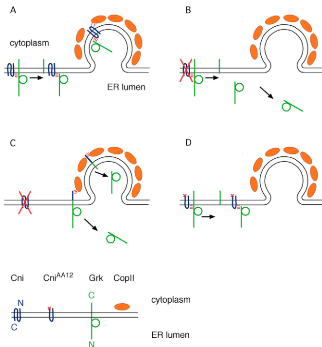
Fig. 9. Schematic representation of Cni function. (A) Wild-type situation. Grk protein binds to Cni after processing in the ER and the released growth factor is recruited into COPII coated vesicles by Cni. (B) In the absence of Cni, processing still occurs but the released growth factor is lost into the ER lumen. (C) Loss of Cni can be partially overcome by fusion of Grk with a COPII targeting motive from Cni or dEmp24. Processing will preferentially occur near ER exit sites, locally increasing the concentration of the soluble growth factor. (D) The truncated Cni AA12 protein can keep processed Grk at the membrane, but fails to efficiently recruit it into outgoing vesicles.
