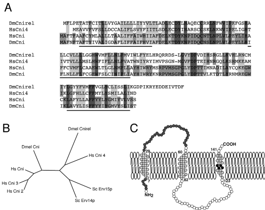
Fig. 3. Cornichon belongs to a conserved protein family. (A) Drosophila Cni and Cni-related, and their human homologues HsCni (gb| AAD20960.1) and HsCni4 (gb| NP_054903.1) share 21.5% identical (dark grey) and 43.9% similar (light grey) amino acids. Conservation is much higher between pairs of homologues: 66.7% identical/85.4% similar in the case of Cni and HsCni, and 51.2% identical/81.8% similar for Cnirel and HsCni4 (residues identical between homologues in medium grey). Conserved residues are distributed along the entire length of the proteins, predicted transmembrane domains are underlined. (B) Rootless phylogenetic tree for the fly, human and yeast Cni family members. Cnirel and human Cni4 form a distinct branch. Tree constructed by neighbour-joining, bootstrap support >98% for all nodes. (C) Model of the membrane topology predicted for Cni using TMHMM ( www.cbs.dtu.dk/services/TMHMM ) and Tmpred ( www.ch.embnet.org ), with the N terminus facing the cytoplasm. The three transmembrane domains are labelled in light grey, while the Grk-binding domain (dark grey) maps to the N terminus, including the first luminal loop. Black residues denote the conserved diaromatic motive.
