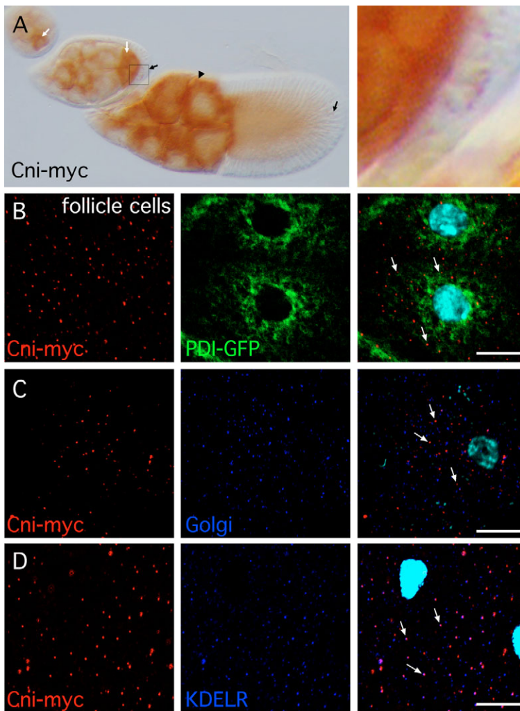
Fig. 2. Cni protein localization. (A) Myc-tagged Cni (Cni-myc) expressed from the endogenous promoter accumulates in the oocyte during early and middle oogenesis (white arrows). At stage 10, strong expression in the nurse cells indicates maternal loading (arrowhead). The protein is also detectable in the somatic follicular epithelium (black arrows). Right panel, magnification of boxed area. (B) C-terminally myc-tagged Cni protein (Cni-myc, red) expressed in the squamous follicle epithelium forms discrete punctate structures, that are often associated (arrows) but not necessarily tightly colocalized with the large reticulate ER of these cells labelled with PDI-GFP (green). (C) Cni-myc (red) does in most cases (arrows) not colocalize with the punctate and disperse Golgi apparatus of the same cells, marked by the p120 Golgi protein (blue). (D) Cni-myc containing structures (red) are largely co-stained (arrows) with an antibody against the KDELR receptor (blue). This protein cycles between ER and Golgi. The total pool of KDELR-receptor positive structures exceeds that co-staining with Cni-myc. (B-D) DNA (DAPI) is shown in light blue. Scale bars: 10 \mu m.
