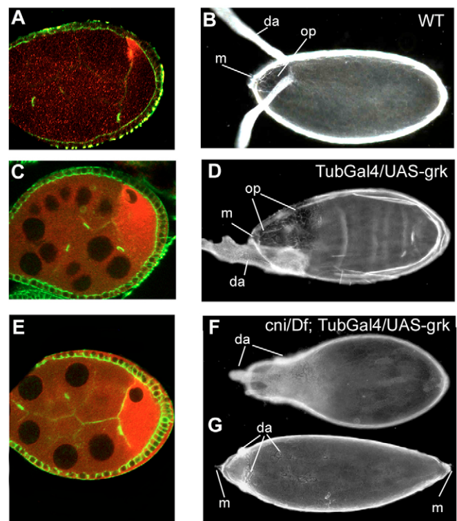
Fig. 8. Gal4-mediated Grk overexpression in the germline can overcome the secretion block in cni ovaries. (A) Wild-type egg chamber. Endogenous Grk (red) is tightly localized to the dorsal anterior corner of the oocyte. Cells are outlined with Phalloidin (green). (B) Wild-type egg. The dorsalmost chorion structure is the operculum (op). Dorsal appendages (da) are derived from more lateral positions. (C,D) Grk overexpression in a wild-type background using the maternal tubulin:Gal4-VP16 driver. (C) Despite a massive increase in the amount of Grk protein, there is still a Grk gradient within the oocyte with highest levels close to the oocyte nucleus. (D) The eggs maintain DV polarity although they have an expanded operculum (op) and the dorsal appendages (da) are shifted to the ventral side. (E-G) Overexpression of Grk in a cni AR55 / Df(2R)H60 background using the maternal tubulin:Gal4-VP16 driver line. (E) High amounts of Grk protein are evenly distributed within the oocyte. (F) The eggs lack DV polarity, but the presence of dorsal appendage material (da) and the suppression of a posterior micropyle indicate low levels of Grk signalling. (G) Despite formation of dorsal appendage material (da), 30% of the eggs lack anteroposterior polarity as can be seen from the presence of a posterior micropyle (m). This indicates a lack of temporal control of Grk signalling.
