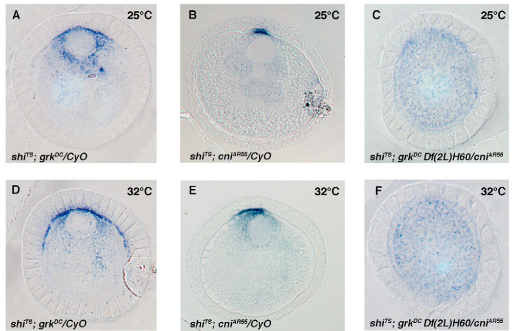
Fig. 5. Trapping of Grk DC protein at the plasma membrane through inactivation of the Drosophila Dynamin homologue Shibire requires Cni function. (A) shi TS ; grk DC /CyO egg chamber incubated at the permissive temperature (25°C). Grk staining at the membrane is limited to the vicinity of the nucleus. Ovaries preincubated in Schneider's medium exhibit higher than usual background, irrespective of their genotype. (B) shi TS ; cni AR55 /CyO egg chamber incubated at 25°C. Grk is distributed in the wild-type pattern. (C) shi TS ; cni AR55 /grk DC Df(2L)H60 egg chamber incubated at 25°C. Grk is diffusely distributed throughout the oocyte. (D) Incubation at 32°C blocks endocytosis in shi TS ; grk DC /CyO oocytes. Membrane tethered Grk DC protein accumulates at the oolemma. (E) Blocking endocytosis in shi TS ; cni AR55 /CyO ovaries has no effect on the wild-type Grk protein not anchored to the oocyte plasma membrane. (F) shi TS ; cni AR55 /grk DC Df(2L)H60 egg chamber incubated at the restrictive temperature. In the absence of cni , Grk DC protein cannot be trapped at the plasma membrane but remains mislocalized to the interior of the oocyte.
