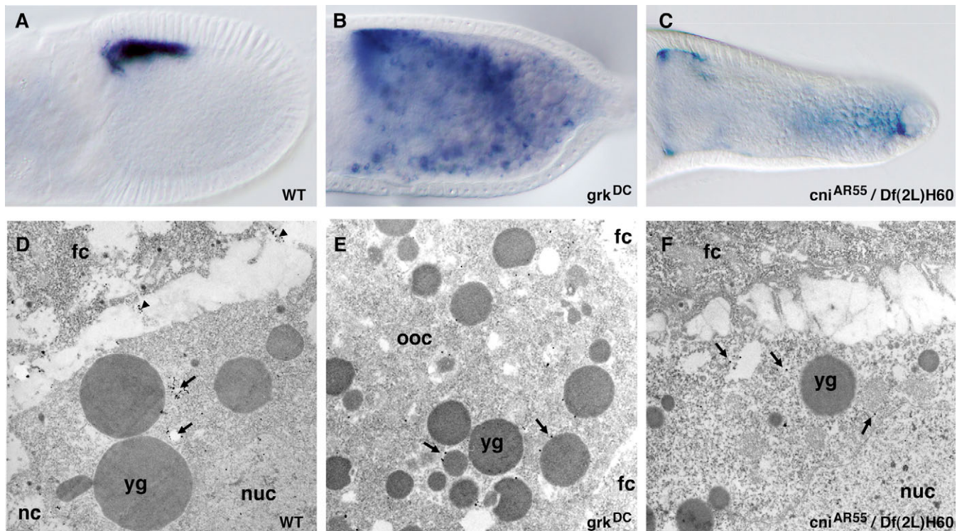
Fig. 4. Grk protein distribution in wild-type, grk DC and cni mutant egg chambers. (A) Stage 10 wild-type egg chamber. Grk protein is concentrated at the anterodorsal corner of the oocyte in the vicinity of the nucleus. Some Grk can be seen in the follicle cells receiving the Grk signal. (B) Stage 10 grk DC /grk DC egg chamber. Grk protein is mislocalized to the interior of the oocyte. The staining appears patchy and granular, with high protein concentration near the nucleus. Grk is not detectable in the follicular epithelium. (C) Stage 10 cni AR55 /Df(2L)H60 egg chamber. Grk protein is distributed in a gradient with a high point near the posteriorly mislocalized oocyte nucleus and in a cortical ring at the anterior end of the oocyte adjacent to the nurse cells. There is no detectable Grk uptake into the follicular epithelium. (D) Immunoelectron microscopy of the anterodorsal corner of a stage 10 wild-type egg chamber. Grk immunogold staining (small black dots) can be detected in the oocyte (ooc) near the nucleus (nuc, arrows) and at the plasma membrane facing both follicle cells (fc) and nurse cells (nc). Grk is also present at the microvillous processes of the follicle cell surface (arrowheads) and within the follicle cells. Grk is absent from the cortex of yolk granules (yg). (E) Immunoelectron microscopy of the ventral posterior part of a heterozygous stage 10 grk DC /CyO oocyte. Most Grk staining is associated with the cortex of growing yolk granules (arrows). (F) Immunoelectron micrograph of a stage 10 cni AR55 /Df(2L)H60 egg chamber. Grk staining is found scattered throughout the oocyte (arrows) but does not accumulate at yolk granules or the oolemma.
