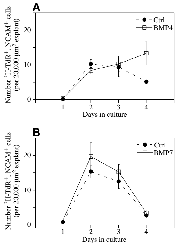
Fig. 8. Low-dose BMP4 promotes survival of newly-generated ORNs. OE explants were cultured in LCM + 1 medium for a total of 96 hours, in the absence of BMP4 or presence of BMP4 (0.1 ng/ml) or BMP7 (1 ng/ml). 16 hours after plating, cultures were pulsed with 3 μCi/ml [ 3 H]thymidine for 4 hours, then either fixed or chased with fresh medium containing 50 μM cold thymidine. At 1 day intervals, cultures were fixed and processed for NCAM immunostaining and autoradiography. To calculate survival of ORNs generated from [ 3 H]thymidine-labelled progenitors, the total number of migratory cells that were doubly positive for [ 3 H]thymidine and NCAM was counted for individual explants at each timepoint in each condition, and that number divided by the explant area. For comparison, labelling indices were normalized to an average explant area of 20,000 μm 2 . Data are graphed as mean ± s.e.m. for 20 explants analyzed in each condition at each timepoint. (A) A significant difference in the numbers of surviving ORNs was observed between control and BMP4-treated cultures at day 4 ( P=0.02 , Student's t -test; Glantz, 1992). (B) BMP7 had no significant effect on ORN survival.
