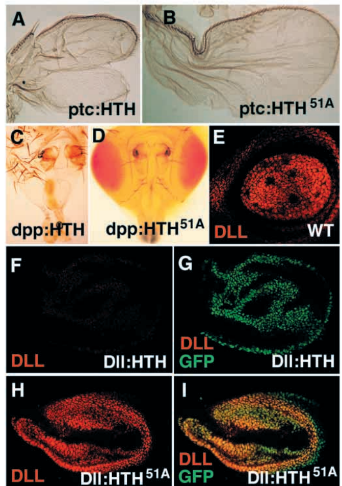
Fig. 3. The HTH homeodomain is required for HTH activity. (A,B) Adult wings resulting from ectopic expression of GFP-HTH (A) or GFP-HTH 51A (B) using the ptc:Gal4 driver line. The wing is split in A. (C,D) Adult heads resulting from ectopic expression of GFP-HTH (C) or GFP-HTH 51A (D) using the dpp:Gal4 driver line. Eyes are completely absent in C. (E-I) Leg imaginal discs in which GFP-HTH (F,G) or GFP-HTH 51A (H,I) were ectopically expressed using the Dll:Gal4 driver line. E shows a wild-type disc for comparison. The discs were stained for DLL (red) and GFP (green); E,F,H show only the red channel and (G,I) show both channels. Expression of GFP-HTH represses Dll expression (F,G), but expression of GFP-HTH 51A does not repress DLL (H,I).
