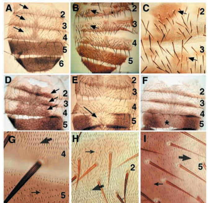
Fig. 6. Altering hth activity affects abdominal segment identity. Shown are dorsal views of adult male abdomens; the numbers on the right in each panel refer to the tergite. (A,G) Wild type; (B,C,H) abdomens with hth - clones (arrows in B,C) marked with y - ; (D) pnr:Gal4 ; UAS-GFP-HM; (E,I) pnr:Gal4 ; UAS-MYC-HTH; (F) pnr:Gal4 ; UAS-GFP-HTH 51A . (A) In wild-type males the anterior two-thirds of tergites 2, 3 and 4 (arrows) are lightly pigmented whereas tergites 5 and 6 are darkly pigmented. Reducing hth activity in tergites 2, 3 or 4 by mosaic analysis (B,C) or by expressing GFP-HM (D) resulted in darkly pigmented cuticle, typical of a posterior tergite identity (arrows). Expression of MYC-HTH (E) resulted in a transformation of tergites 5 and 6 into a more anterior, lightly pigmented identity (arrow); GFP-HTH generates an identical transformation (not shown). GFP-HTH 51A is also weakly able to produce this transformation (F, asterisk). In D-F the transformations are observed in a dorsal band of cells, which is where the pnr:Gal4 driver is expressed (Calleja et al., 1996). (G) In addition to differences in pigmentation, anterior tergites (e.g. tergite 4; large arrow) also have a higher density of trichomes, or small hairs, than posterior tergites (e.g. tergite 5, small arrow). (H) hth - clones in anterior tergites have a lower density of trichomes (small arrow) than the surrounding wild-type cuticle (large arrow), indicating a transformation to a more posterior identity. (I) A close-up of the border between MYC-HTH-expressing cells (lighter pigmented region on the right) and wild-type cells (darker pigmented region on the left) in tergite 5. In addition to affecting pigmentation, expression of MYC-HTH in posterior segments also resulted a higher density of trichomes (large arrow). Expression of GFP-HM did not affect trichome density, suggesting that the reduction of hth activity is incomplete (not shown). In G-I large and small arrows point to regions of higher and lower trichome density, respectively.
