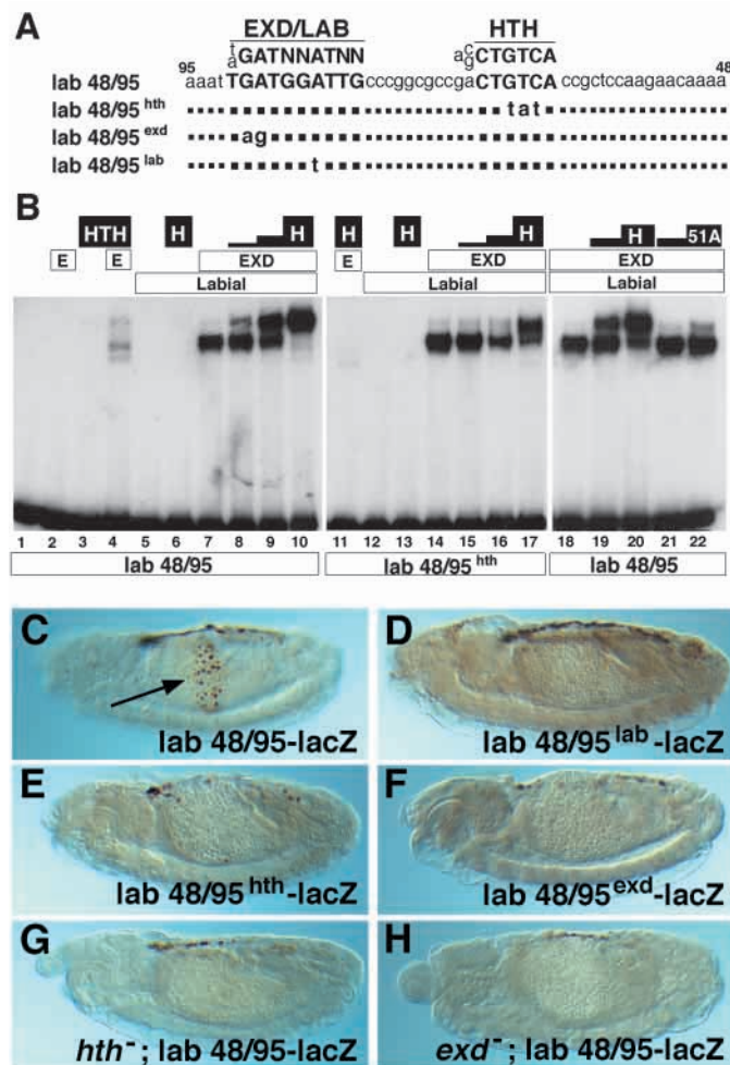
Fig. 4. HTH, LAB and EXD form an essential complex on the Hox target, lab48/95 . (A) Sequence of lab48/95 and mutant derivatives. The EXD/LAB and HTH binding sites are indicated in bold; mutations are indicated in small letters. For comparison, the Hox/EXD and MEIS1 consensus binding sites are shown above the lab48/95 sequence (Mann and Chan, 1996; Chang et al., 1997). (B) Band shift experiments using 32 P-labelled lab48/95 (lanes 1-10 and 18-22) and lab48/95 hth (lanes 11-17) oligos. Neither EXD (lane 2) nor HTH (lane 3) bind this DNA on their own. When EXD and HTH (H) are combined they form a weak complex (lane 4). Neither LAB (lane 5) or a mixture of LAB plus HTH (lane 6) bind this DNA. In contrast, LAB plus EXD bind to this DNA (lane 7) and increasing amounts of HTH shift this band to a slower migrating, HTH/LAB/EXD complex (lane 8-10). On lab48/95 hth EXD plus HTH bind very poorly (lane 11), but LAB plus EXD bind as well as on lab48/95 (lanes 7 and 14). Upon addition of increasing amounts of HTH, a HTH/LAB/EXD band forms only at the highest HTH concentration (lane 15-17). In the right-most panel, HTH is able to supershift the LAB/EXD complex (lanes 19-20) whereas the same concentrations of HTH 51A (51A) resulted in only a very weak supershift (lanes 21-22). As indicated, the amounts of HTH and HTH 51A in lanes 19 and 21 are intermediate to the amounts of HTH in lanes 8 and 9; similarly, the amounts in lanes 20 and 22 are intermediate to the amounts in lanes 9 and 10. (C-H) lab48/95 requires exd , hth and the LAB, EXD and HTH binding sites. Transgenic embryos were immunostained for \beta -gal and detected using HRP (brown). In wild-type lab48/95-lacZ embryos (C) strong nuclear staining is observed in a central band of endoderm cells (arrow); staining is absent in hth - (G) or exd - (H) embryos. lab48/95 activity also requires lab (Grieder et al., 1997). No endoderm staining is observed when the EXD (F) or LAB (D) binding sites are mutated, and is very weak when the HTH binding site is mutated (E). Dorsal staining, unrelated to labial expression, is observed in all of these embryos (Grieder et al., 1997).
