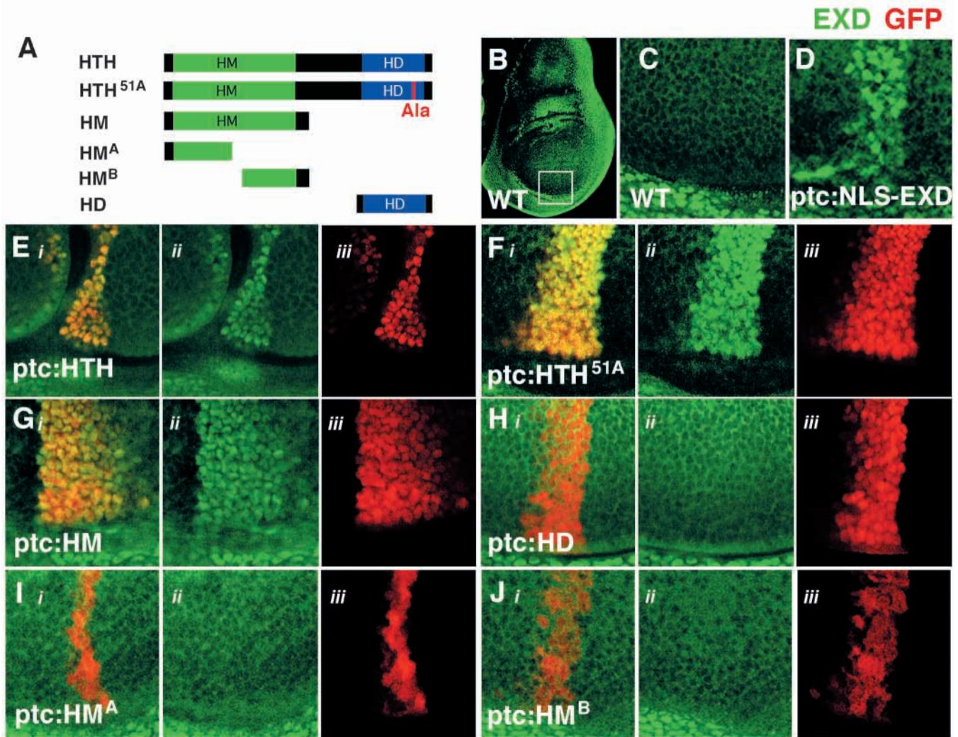
Fig. 2. The HM domain of HTH is necessary and sufficient for the nuclear import of EXD. (A) Schematic diagram of wild-type and mutant HTH proteins, which were expressed in imaginal discs as N-terminal GFP fusion proteins (GFP sequences are not shown). (B,C) A wild-type wing imaginal disc stained for EXD (green) shows cytoplasmic staining in wing pouch cells and nuclear staining in more peripheral regions. The box in B indicates the approximate region shown in C-J. (D) Confocal micrograph showing expression of NLS-EXD using the ptc-Gal4 driver line and stained for EXD protein (green). NLS-EXD, which has an additional NLS fused to the N terminus, is predominantly nuclear in the absence of HTH. (E-J) Confocal images of wing discs ectopically expressing GFP-HTH variants using the ptc:Gal4 driver. The discs were stained for EXD (green) and GFP (red) to detect the GFP-HTH variants. The i panels show the double images and the ii and iii panels show individual green or red channels, respectively. Endogenous EXD is imported into nuclei by GFP-HTH (E), GFP-HTH 51A (F), and GFP-HM (G), but not by GFP-HD (H), GFP-HM A (I), or GFP-HM B (J). GFP-HM (Giii) and GFP-HD (Hiii) are nuclear, GFP-HM A is present in both the nucleus and cytoplasm (Iiii) and GFP-HM B is predominantly detected in the cytoplasm (Jiii). GFP-HM A or GFP-HM B could also be detected with an anti-HTH antibody (not shown), confirming the presence of HTH sequences in these fusion proteins. Note also that ptc -driven expression of HTH induces a fold in the wing pouch (E) whereas the other HTH derivatives do not, indicating that HTH must be competent to bind DNA to induce this morphological change.
