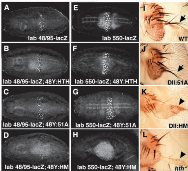
Fig. 5. The HM domain interferes with hth function. lab48/95 (A-D) or lab550 (E-H) expression in wild-type embryos (A,E) and embryos expressing GFP-HTH (B,F), GFP-HTH 51A (C,G), or GFP-HM (D,H) using the endodermal Gal4 driver line, 48Y:Gal4 . Compared to wild-type levels (A,E), GFP-HTH (B,F) or GFP-HTH 51A (C,G) expression had no effect on \beta -gal levels, whereas GFP-HM expression reduced or eliminated \beta -gal levels (D,H). In A-H \beta -gal was detected by immunofluorescence. (I-L) Adult antennae. A wild-type antenna (I), antennae in which GFP-HTH 51A (J) or GFP-HM (K) were expressed using the Dll:Gal4 driver, and an antenna with a distal hth - clone, identified by yellow - tissue (L). In both (K) and (L) a transformation of distal antenna towards distal leg was observed (arrowheads). The antennae in I and J are wild type (arrows).
