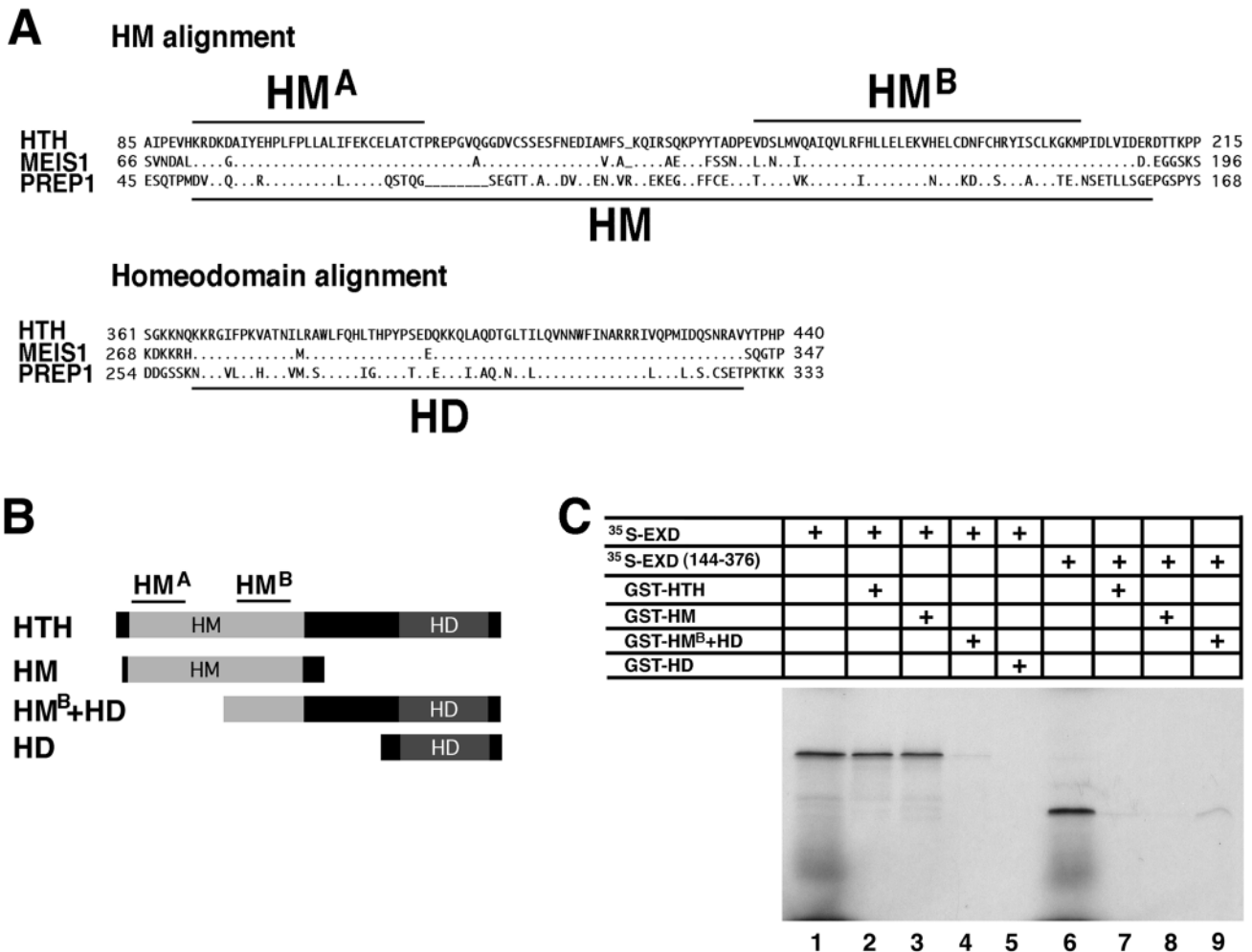
Fig. 1. HTH binds to EXD via its HM domain. (A) Sequence alignments of the HM and homeo domains of HTH, MEIS1 and PREP1. The two subregions of the HM domain that are conserved in PREP1 are referred to here as HM A and HM B . (B) Schematic diagram of HTH deletion constructs. All HTH proteins were synthesized in E. coli as N-terminal GST fusion proteins (GST sequences are not shown). (C) GST pull down experiment with the fusion proteins depicted in B and 35 S-labeled EXD proteins. Lanes 1 and 6 show 25% of the 35 S-EXD and 35 S-EXD[144-376], respectively, that was used in the binding reactions. GST-HTH (lane 2) and GST-HM (lane 3) bind approximately 25% of the input 35 S-EXD, whereas GST-(HM B +HD) (lane 4) and GST-HD (lane 5) do not bind 35 S-EXD in this assay. 35 S-EXD[144-376], which lacks the PBC-A domain of EXD, does not bind any of the HTH derivatives.
