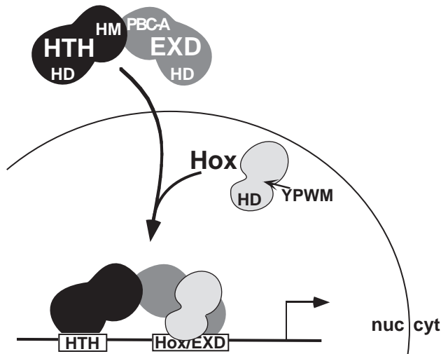
Fig. 7. Formation of a Hox protein complex on a Hox target enhancer. The cytoplasmic to nuclear translocation of EXD requires a direct interaction between the HM domain of HTH and the PBC-A domain of EXD. Once in the nucleus, HTH remains associated with EXD and, together with a Hox protein, can assemble into a Hox protein complex that requires an interaction between the Hox 'YPWM' motif and the EXD homeodomain. The Hox protein complex recognizes DNA via all three homeodomains (HD) with a high degree of sequence specificity. In lab48/95 , HTH binds at a distance from and helps to stabilize the Hox/EXD heterodimer. We suggest that the conserved regions of HTH and EXD are likely to recruit additional proteins to this complex to regulate transcription. nuc, nucleus; cyt, cytoplasm.
