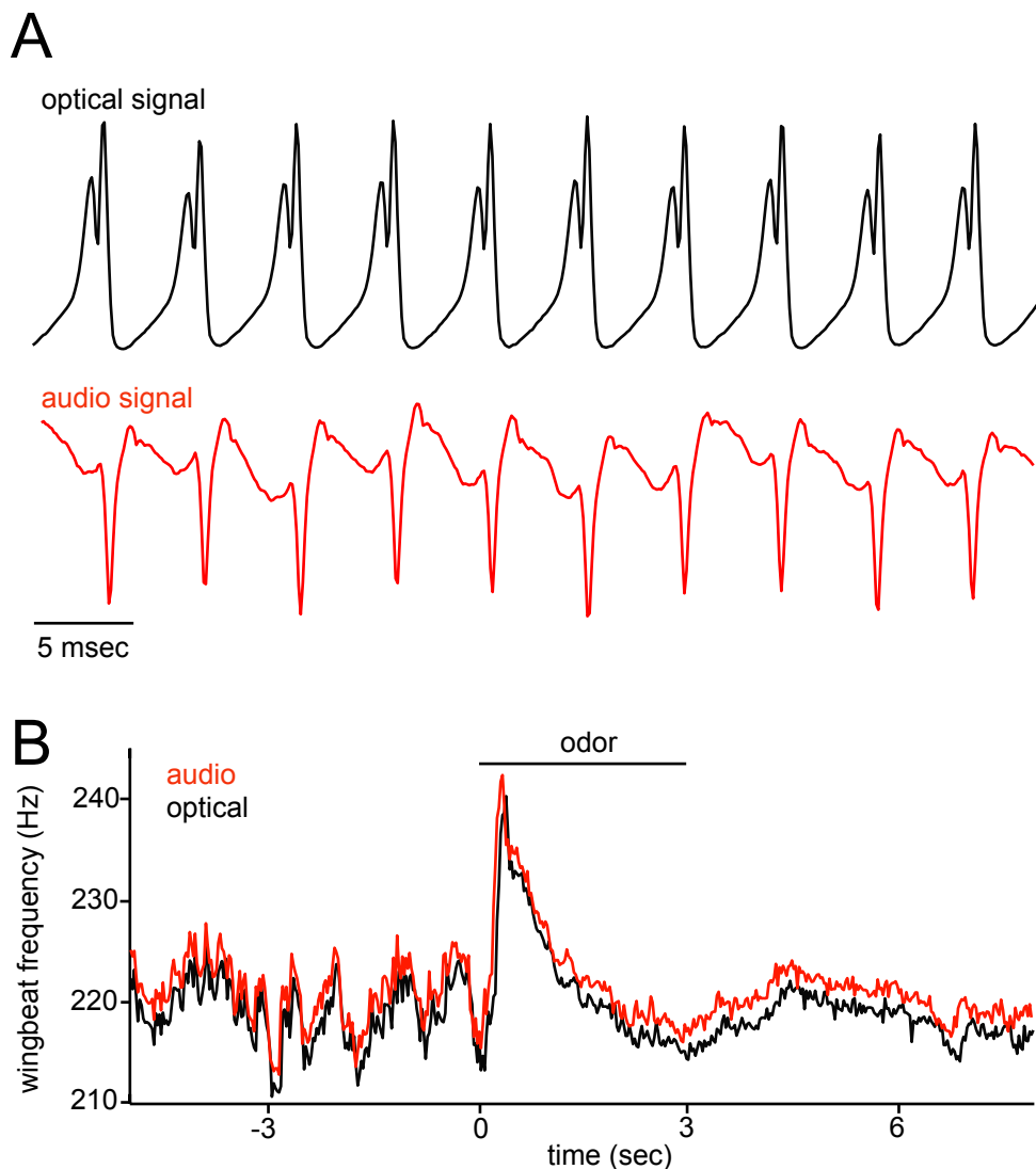
Supplementary Figure 3: Comparison of wingbeat frequency measurements obtained with a photodiode and with a microphone in the rotatable-tether apparatus.
