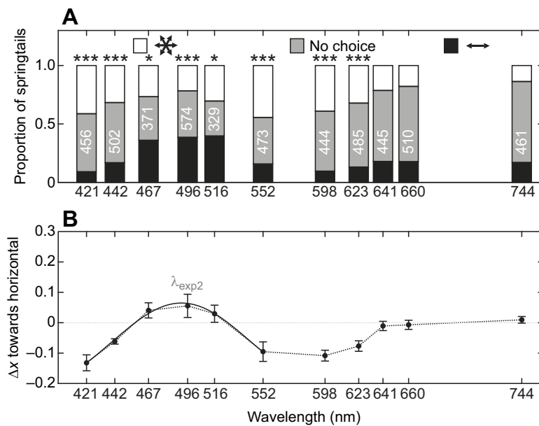
Fig. 7. Response of springtails to horizontally polarized light against unpolarized stimulus as a function of wavelength (experiment 2). (A) Proportion of total springtails in the arena terminals corresponding to the horizontally polarized stimuli (black bars), unpolarized stimuli (white bars) and the inactive specimens in the middle of the arena (gray bars). Total numbers of tested springtails are shown in the gray bars. * P < 0.05 , *** P < 0.0001 , in \chi^2 tests. (B) Mean relative centroid shifts \Delta x of springtails towards horizontally polarized stimulus. Vertical bars represent the s.e. of the 4 trials. Gaussian function fitted on the 421–552 nm region is shown by solid line. Wavelength of Gaussian maximum is \lambda_{\text{exp2}} = 491 nm.
