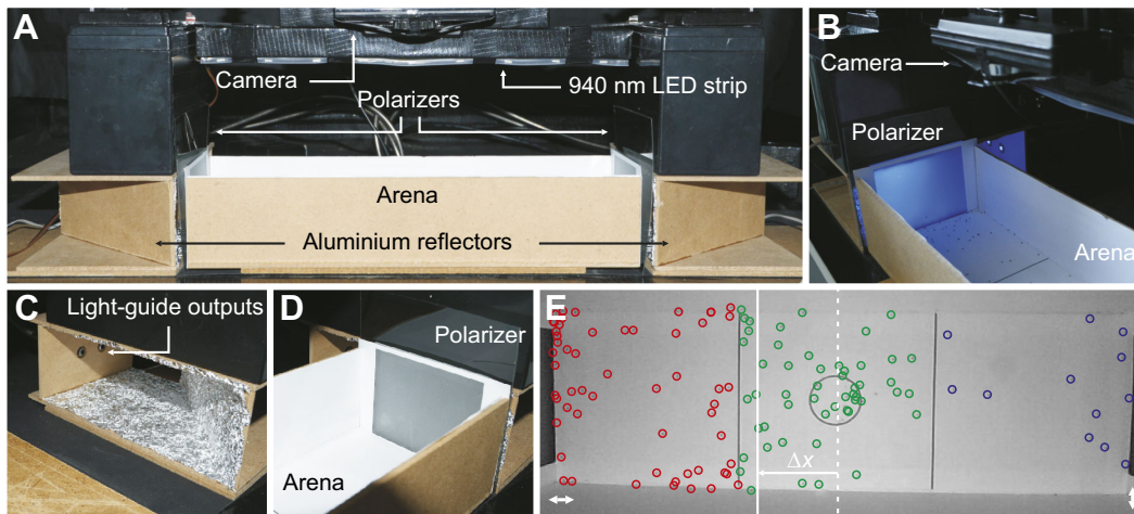
Fig. 4. Measurement of the wavelength dependence of polarotaxis. (A) Photograph of the experimental setup used for experiments 2 and 3. (B) Setup with a horizontally polarized blue stimulus ( \lambda_{\text{stimulus}}=442 nm). (C) Aluminium reflector used to diffusely reflect light from the light guide outputs. (D) Arena in position in front of the reflector. (E) Example of the detection of springtails for a horizontally/vertically (left/right) polarized stimulus pair in experiment 2 ( t=70 s, \lambda_{\text{stimulus}}=496 nm). Relative centroid shift of springtail \Delta x towards horizontally polarized stimulus calculated as in Fig. 3B.
