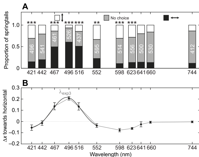
Fig. 8. Response of springtails to equal-intensity stimulus pairs of horizontally and vertically polarized light (experiment 3). (A) Proportion of total springtails in the arena terminals corresponding to the horizontally polarized stimuli (black bars), vertically polarized stimuli (white bars) and the inactive specimens in the middle of the arena (gray bars). Total numbers of tested springtails are shown in the gray bars. ** P < 0.001 , *** P < 0.0001 , in \chi^2 tests. (B) Mean relative centroid shifts \Delta x of springtails towards horizontally polarized stimulus. Vertical bars represent the s.e. of the 4 trials. Gaussian function fitted on the 421–552 nm region is shown by solid line. Wavelength of Gaussian maximum is \lambda_{\text{exp3}} = 492 nm.
