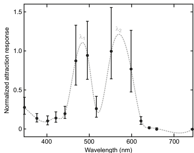
Fig. 6. Action spectrum of phototaxis of P. aquatica . Vertical bars were calculated from the asymptotic standard errors of log photon flux ( J_{50\%} ) needed for eliciting 50% response, and the dashed line shows cubic spline interpolation. \lambda_1 = 484 nm and \lambda_2 = 570 nm are the positions of the two maxima.
