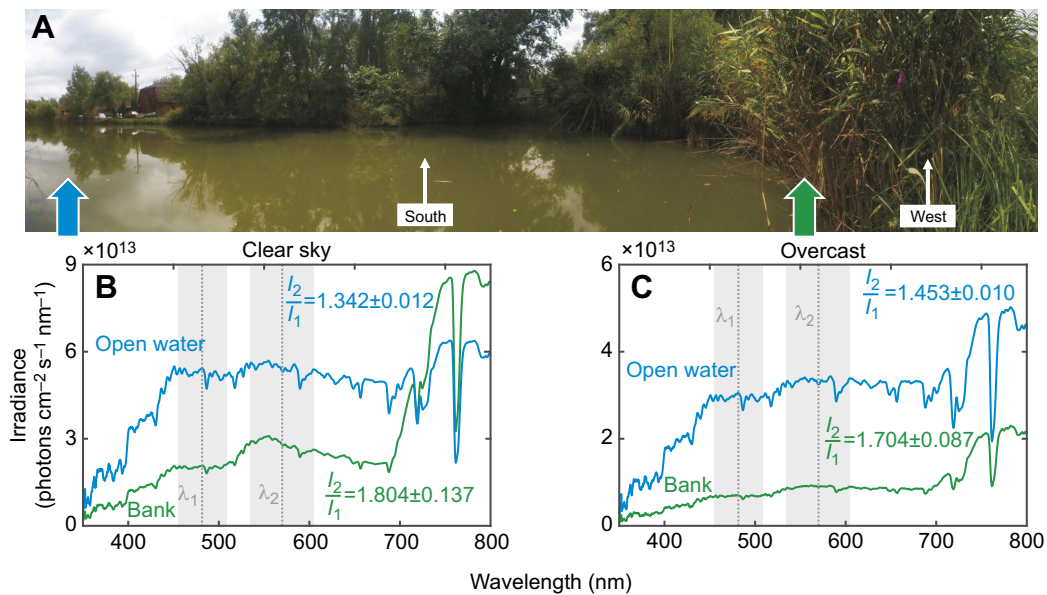
Fig. 9. Spectral characteristics of a natural habitat of P. aquatica . (A) Panorama photo of a small lake from a fishing pier. The arrows represent horizontal measuring directions (blue: towards open water; green: towards bank). (B) Measured spectrum of the sunny environment with spectrometer directed towards the open water (blue) and the bank (green). Gray regions show the FWHM of the two peaks of the action spectrum of phototaxis (Fig. 6). Mean \pm s.d. ratios of integrated photon counts ( I_2/I_1 ) in the regions around \lambda_1 and \lambda_2 are shown with blue (open water) and green (bank) formulas. (C) Measured spectrum under totally overcast conditions.
