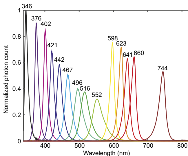
Fig. 2. Emission spectra of the monochromatic light stimuli in case of equal photon flux for each LED. Areas under curves are equal. Numbers show the peak wavelength of each LED.
