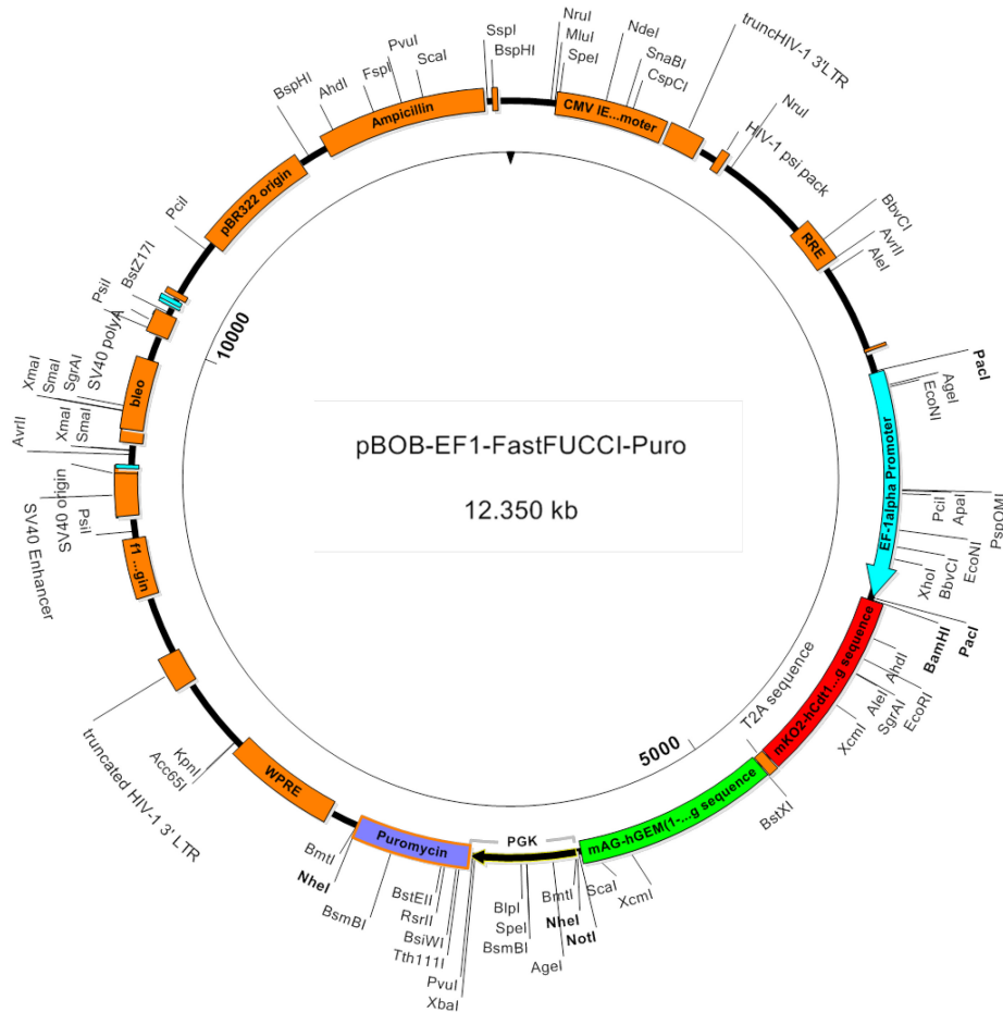
Figure S1, related to Figure 1. pBOB-EF1-FastFUCCI-Puro construct
