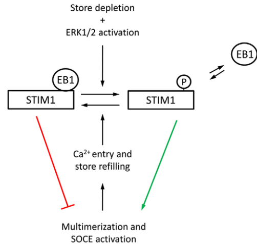
Fig. 8. Regulation of SOCE by phosphorylation of STIM1 at ERK1/2 sites. \text{Ca}^{2+} release from the ER leads to a decreased intraluminal \text{Ca}^{2+} concentration and to ERK1/2 activation. ERK1/2 phosphorylates STIM1 at Ser575, Ser608 and Ser621, triggering the dissociation from EB1. EB1-dissociated STIM1 then aggregates to form puncta, which is a prior step for the activation of SOC channels. Refilling of \text{Ca}^{2+} stores facilitates STIM1 dephosphorylation, thus enhancing STIM1-EB1 binding to avoid prolonged STIM1-dependent activation of SOC channels.
