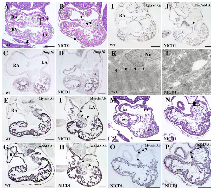
Fig. 2. Morphological and histological defects induced by NICD1-activation. (A,B) Sections stained with Hematoxylin and Eosin show normal EMT in the AV cushion (brackets) and trabecular development in wild-type hearts (A), whereas the trabeculae are not formed normally in NICD1-activated hearts (B). Ectopic cell masses were also evident (arrowheads in B), the interventricular septum is right-shifted (arrow) and trabeculation occurs in the AV myocardium (asterisk in B) in NICD1-activated hearts. (C,D) Bmp10 expression was observed in the trabecular cells in both the wild-type (C) and NICD1-activated (D) ventricles. (E-J,O,P) Immunohistochemistry using anti-myosin (E,F,O), anti- \alpha -smooth muscle actin ( \alpha Sma) (G,H,P) and anti-Pecam (I,J) antibodies reveal that ectopic cell masses (arrowheads) are present in the cushion tissue in NICD1-activated hearts (F,H,J,O,P), but are never observed in wild-type hearts (E,G,I). (M,N) Hematoxylin and Eosin staining at E9.5 also shows ectopic cell masses in the cushion of NICD1-activated heart (arrowheads in N) but not in wild-type heart (M). (K,L) In wild-type myocardium (K), myofibrils with sarcomere structures (Z bands are indicated by black arrowheads) are observed by transmission electron microscopy, but only thin myofibrils without a proper sarcomere structure (no Z band indicated by white arrowheads) are formed in NICD1-activated hearts (L). Embryo samples were prepared at either E10.5 (A-L) or E9.5 (M-P). Serial sections were used for E,G,I (wild-type), F,H,J (NICD1-activated) and N-P (NICD1-activated). Abbreviations: LA, left atrium; RA, right atrium; LV, left ventricle; RA, right ventricle; Nu, nucleus. Scale bars: 200 \mu m in A-J,M-P; 1 \mu m in K,L.
