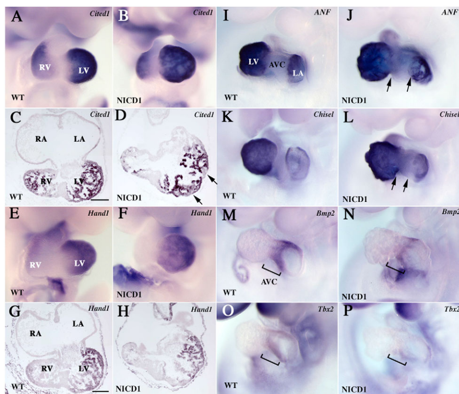
Fig. 3. Molecular characterization of defects in NICD1-activated hearts.
