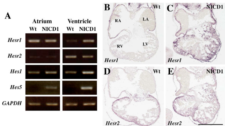
Fig. 4. Expression changes in the Hes and Hesr gene families at E10.5. (A) Semi-quantitative RT-PCR analysis showing upregulation of Hesr1 , Hes1 and Hes5 in NICD1-activated hearts. Hesr1 is ectopically induced at particularly high levels in the ventricle. In situ hybridization analysis also revealed the ectopic induction of Hesr1 in the ventricle and AV canal of NICD1-activated hearts (C), whereas Hesr1 is expressed only in the atrium in wild-type hearts (B). In contrast to Hesr1 , Hesr2 is expressed in the ventricle in wild-type hearts (D) and its distribution is not altered in NICD1-activated hearts (E). Abbreviations: LA, left atrium; RA, right atrium; LV, left ventricle; RV, right ventricle. Scale bar: 500 \mu m in E.
