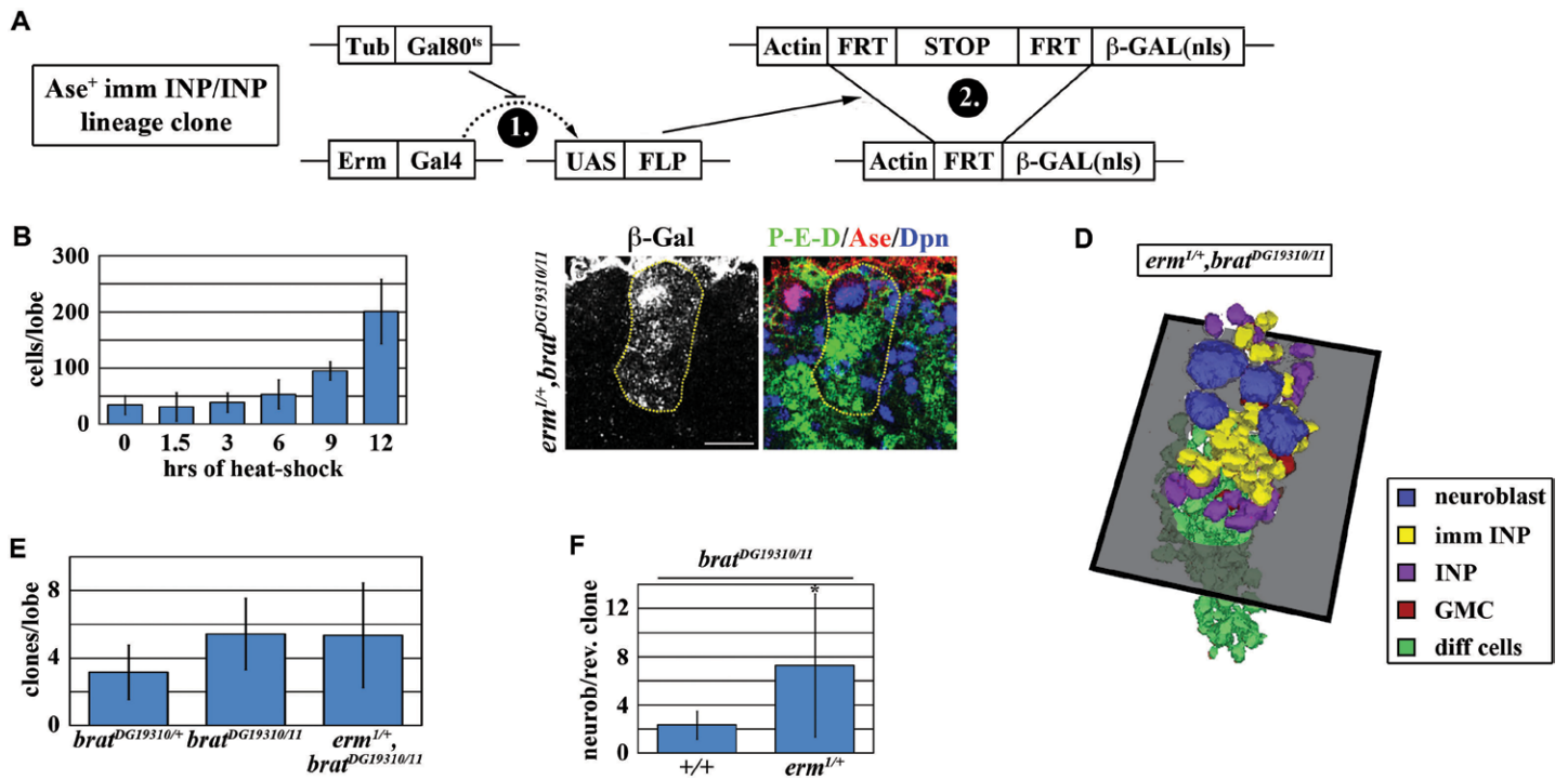
Fig. S2 Empirical determination of the condition required for inducing a low number of clones derived from single Ase + immature INPs or INPs per brain lobe.
