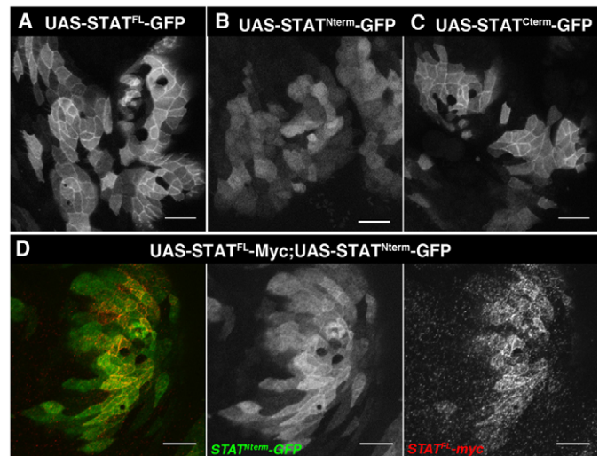
Fig. 2. STAT92E homodimerization and membrane localization domains. (A-C) Ectodermal expression of full-length STAT92E (A), or the N-terminal (B) or the C-terminal (C) half of the protein in germline clone embryos lacking the endogenous STAT92E. In stat92E -null embryos the full-length (A) and C-terminal half (C) localize to the membrane, whereas the N-terminal half (B) is unable to localize to the apical membrane. (D) In this same background, the N-terminal half regains weak apical membrane localization when co-expressed with full-length STAT92E-Myc. (A-C) GFP staining. (D) GFP on the middle and anti-Myc on the right panel with merged channels on the left. Scale bars: 10 \mu m. All pictures are centred in posterior spiracle region. Anterior is leftwards and dorsal is upwards.
