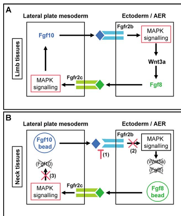
Fig. 8. Interruption of the Fgf feedback loop in the neck. (A) Schematic representation of the Fgf feedback loop that initiates limb budding for a normal limb and for an ectopic limb in the flank; details in the text. (B) In the neck, Fgf signalling is interrupted at distinct points in the neck lateral mesoderm and ectoderm, rendering this region limb-incompetent. Fgfr2b/2c, Fgfr2 IIIb/IIIc.
