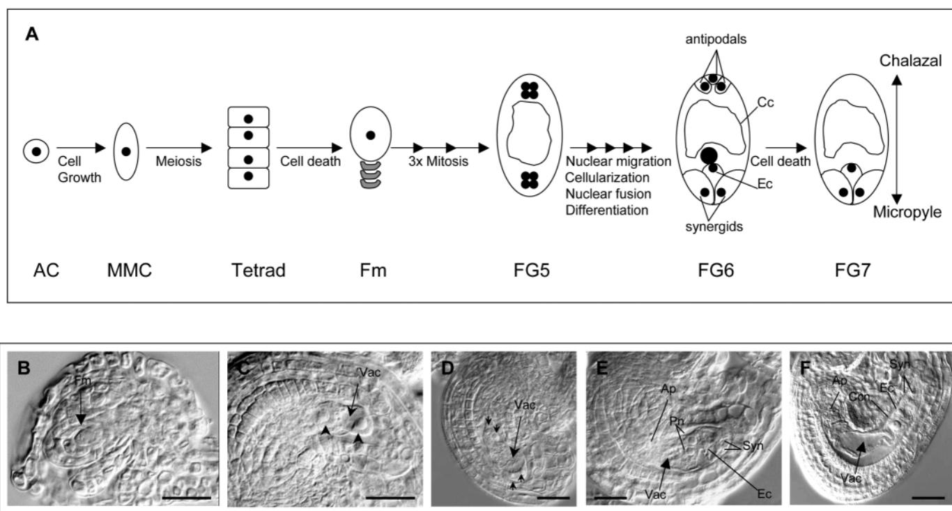
Fig. 1. Wild-type female gametophyte development in Arabidopsis . (A) Scheme showing the sequential developmental events leading to the wild-type female gametophyte formation in Arabidopsis . (B) Wild-type embryo sac containing one functional megaspore. (C) Wild-type embryo sac at the two-nuclear stage. Arrowheads indicate nuclei. (D) Wild-type embryo sac at the four-nuclear stage. Arrowheads indicate nuclei. (E) Cellularized wild-type embryo sac containing eight nuclei. (F) Wild-type embryo sac containing seven cells and seven nuclei. AC, archesporial cell; Ap, antipodal cells; Cc, central cell; Ccn, central cell nucleus; Ec, egg cell; FG5, eight-nuclear embryo sac; FG6, seven-cell embryo sac; FG7, four-cell embryo sac; Fm, functional megaspore; MMC, megaspore mother cell; Pn, polar nuclei; Syn, synergide; Vac, vacuole. Scale bar: 25 \mu m.
